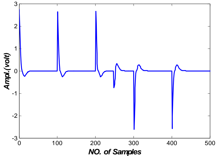
Figure (17) Control action of the FLC with disturbance
