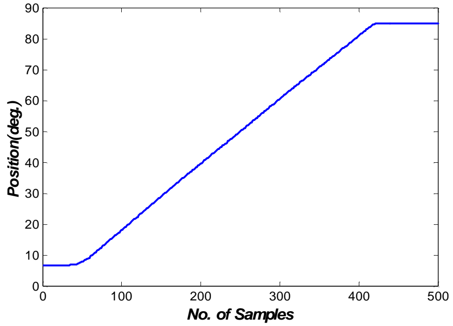
Figure (3) position of the SS exited by a 1-volt step command input
