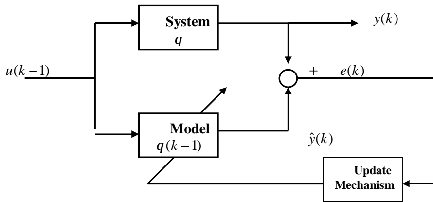
Figure (1) Visualization of Recursive Estimation
