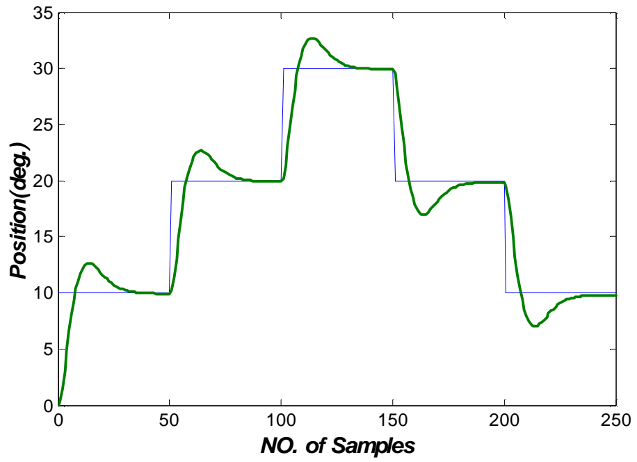
Figure (14) the output of the SS under FLC
