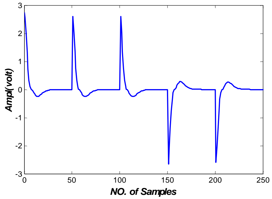
Figure (15) Control action of the FLC
