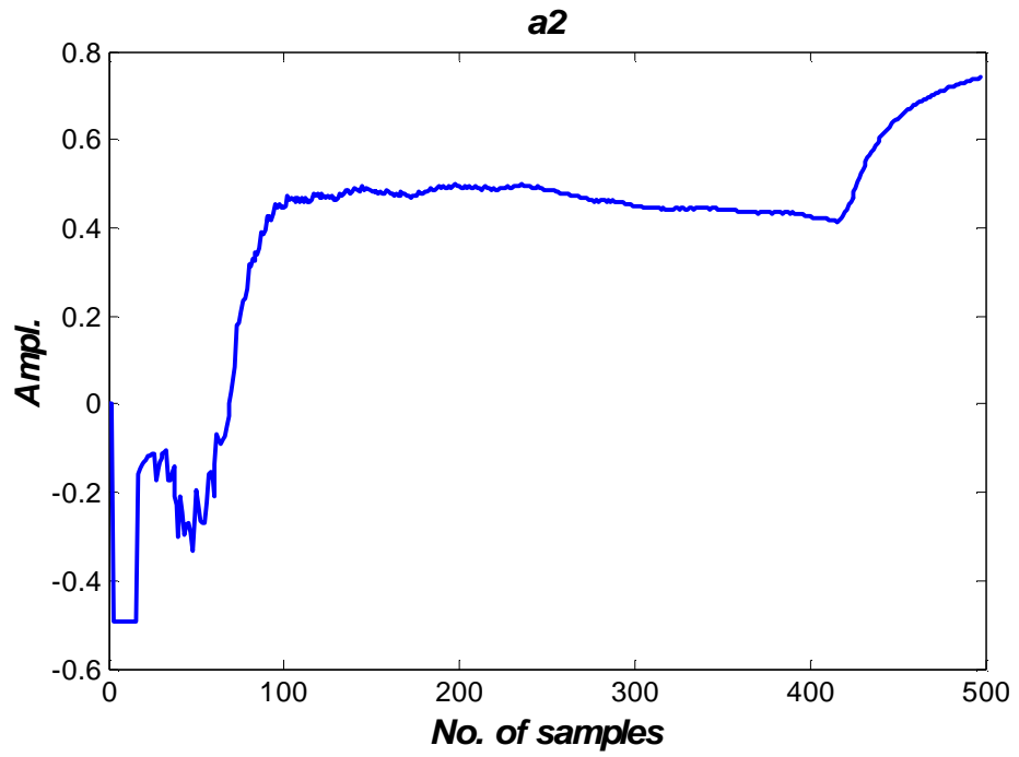
Figure (8) parameter estimate of the RLS
