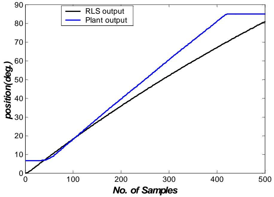
Figure (4) position of the SS exited by a 1-volt step command input and the RLS estimated position exited by the same input.
