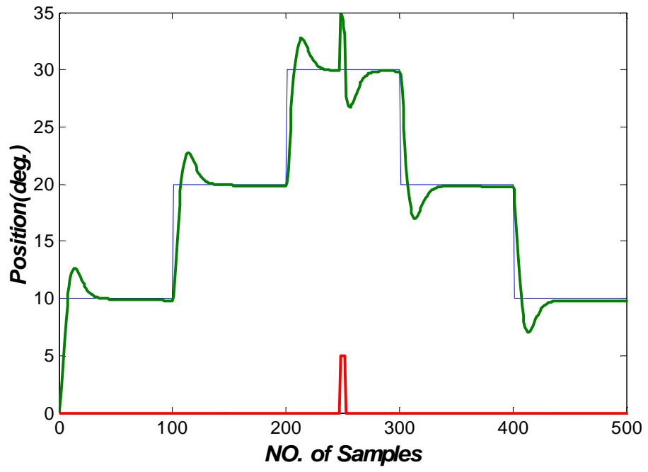
Figure (16) the output of the SS under FLC with disturbance
