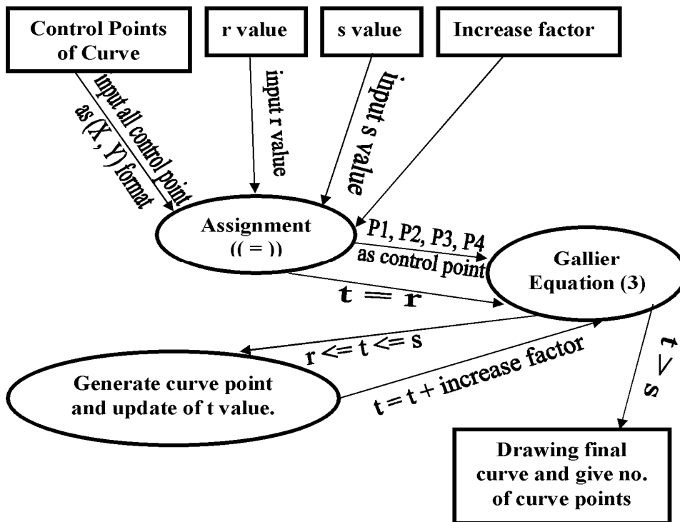
Figure 9: Show top DFD level of proposal work.
