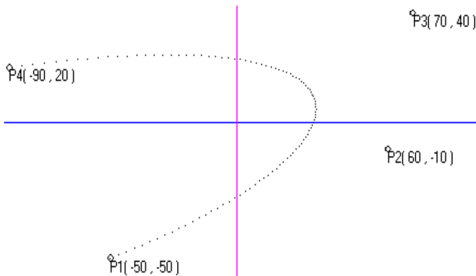
Figure 5: Increase factor =0.01, curves points=100, r=0, s=1,(s-r)=1
