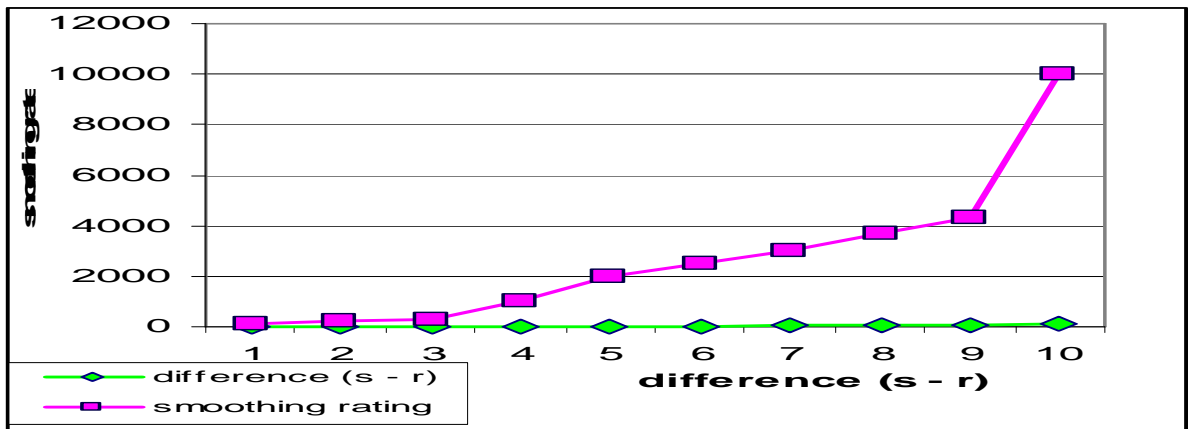
Figure 7: relationships between smoothing with difference s-r in increase factor=0.01
