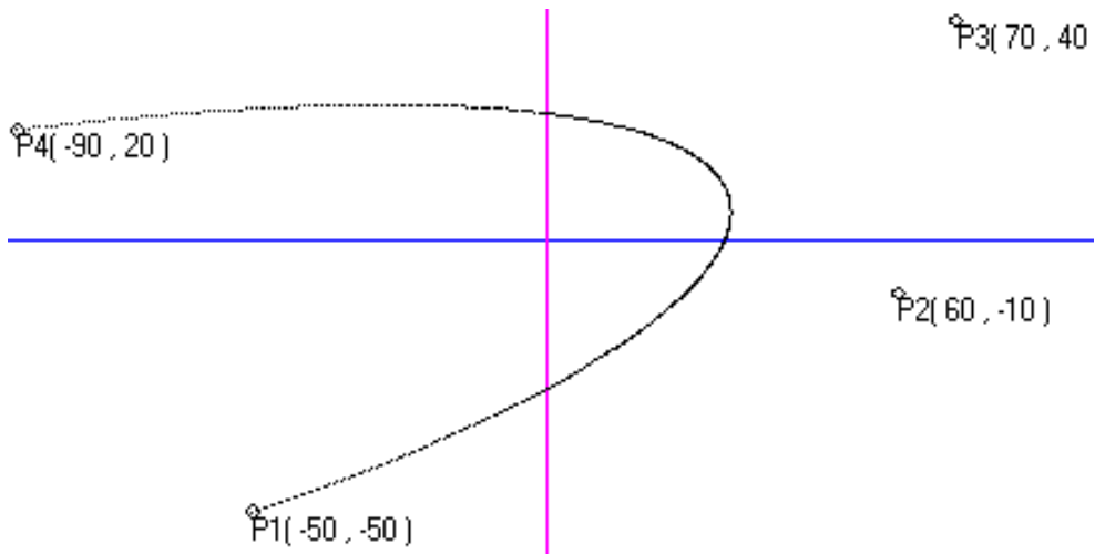
Figure 6: Increase factor =0.01, curves points=501, r=0, s=5, (s-r) =5
