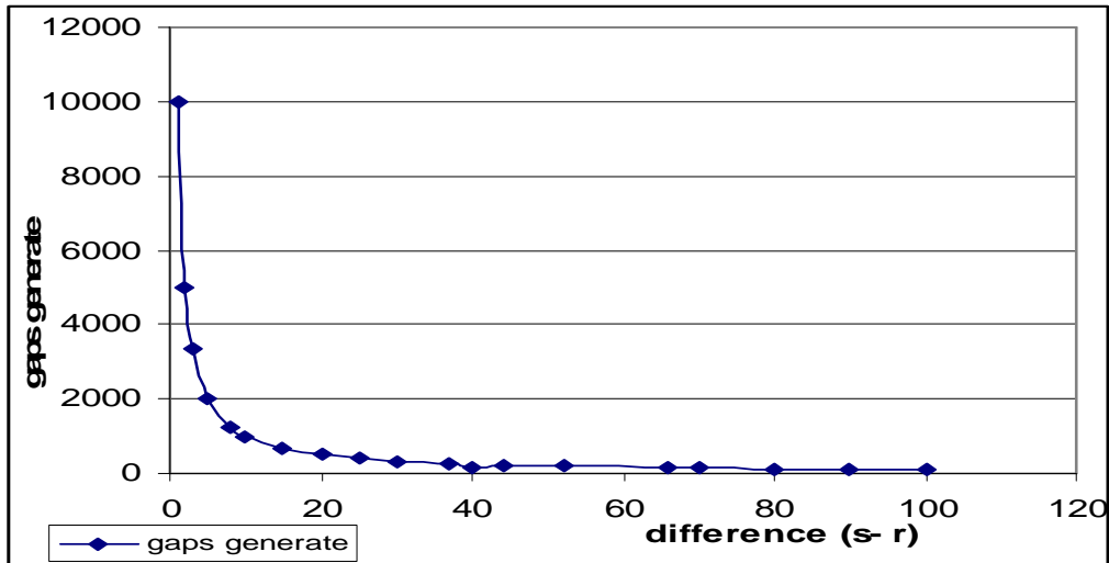
Figure 8: show relationship between gaps curve points with difference s-r in increase factor =0.01
