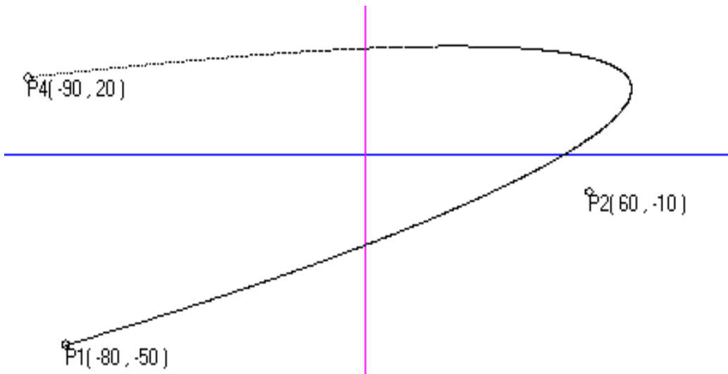
Figure2: Curve smoothing inc. factor =0.001in scattered control points
