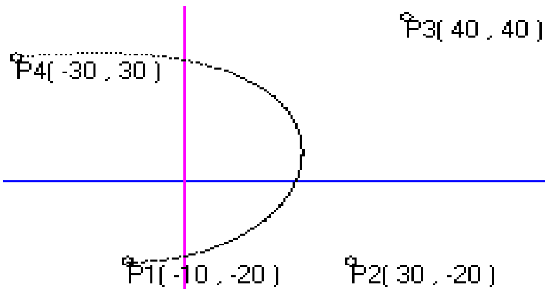
Figure 3: Curve smoothing inc. factor = 0.005 before scaling Bezier curve
