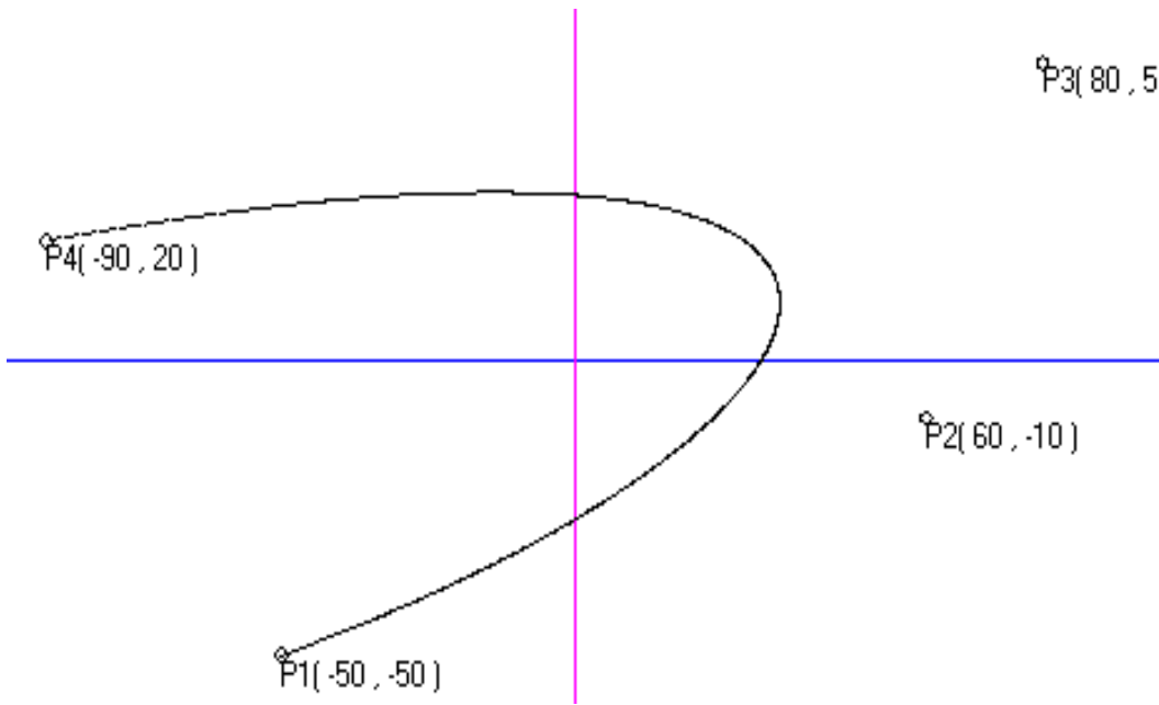
Figure1: Curve smoothing inc. factor =0.001
