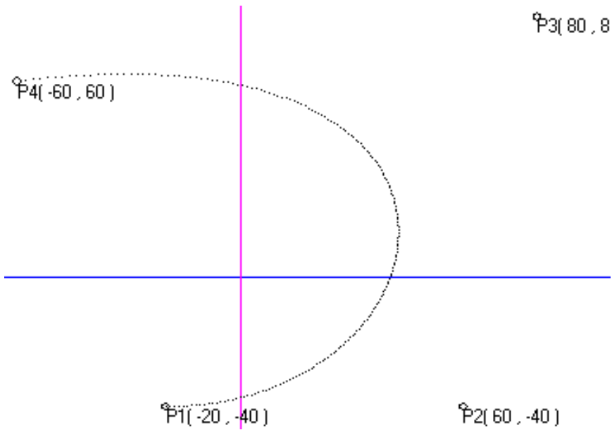
Figure 4: Curve smoothing inc. factor = 0.005 after scaling Bezier curve
