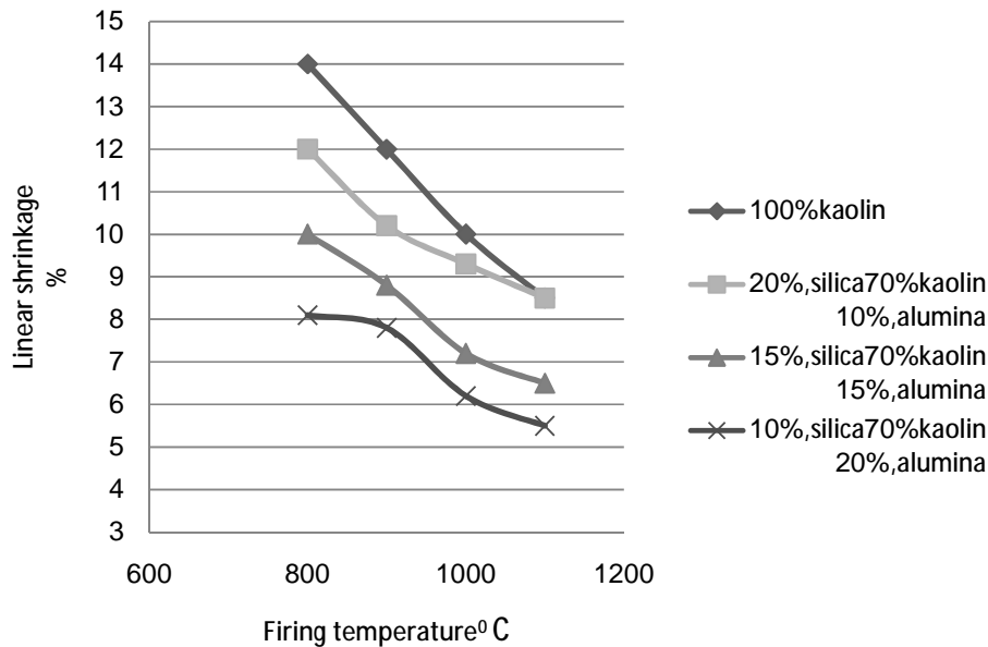
Figure (1) the linear shrinkage of red kaolin with different alumina and silica contained, as a function of firing temperature.
