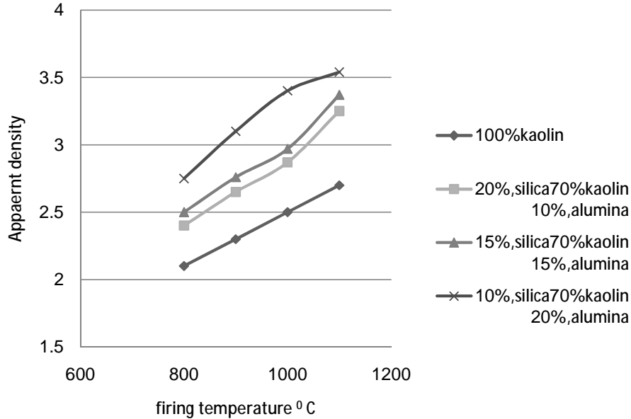
Figure (3) the apparent density of red kaolin with different alumina and silica contained, as a function of firing temperature.
