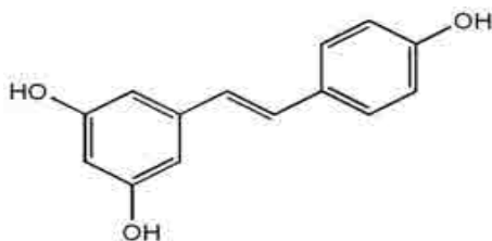
Fig (1) Trans- Resveratrol Structure [17]
