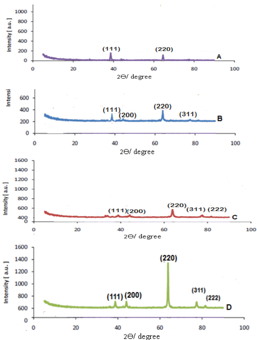
Figure (3). XRD pattern of silver at same conditions.
