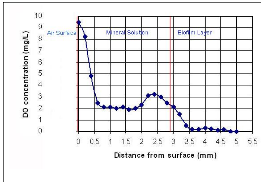
Figure (3): Microprofile of DO concentration measured by MES in an aerobic biofilm with mineral solution.
