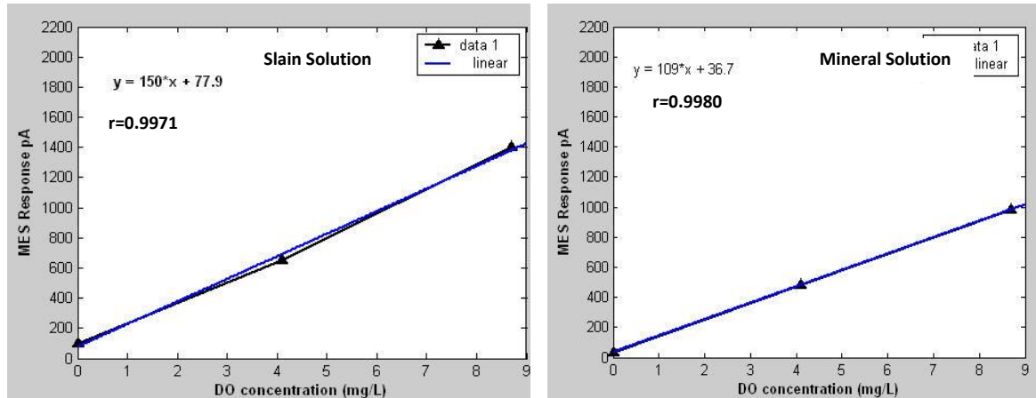
Figure (2): Calibration Graph shown Saline solution (0.85% NaCl solution) and Mineral solution.
