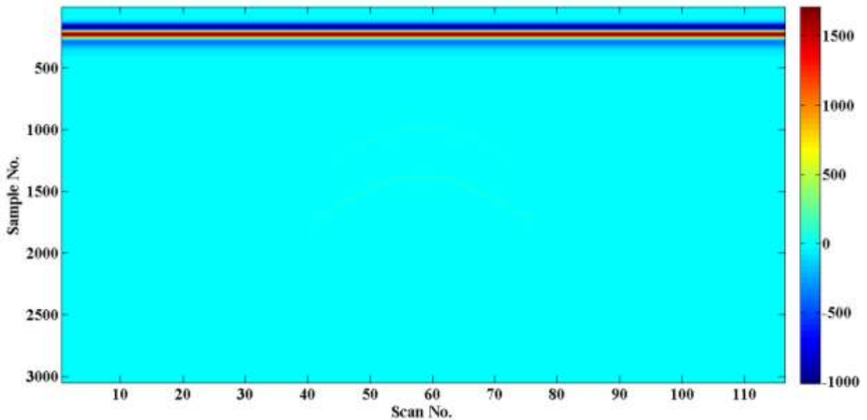
Figure (6):The synthetic results of the clay-filled pipemodel.
