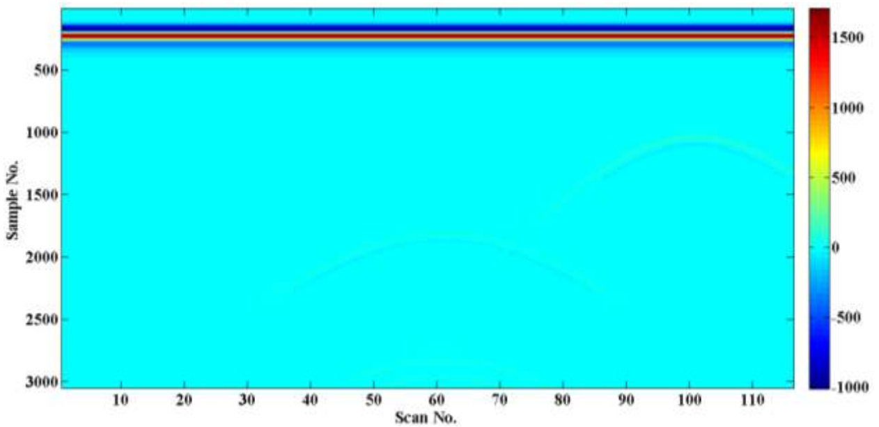
Figure (10):The synthetic results of the fifth model, clay-filled pipe, water-filled pipe, and air-filled pipe have same diameters and placed in different depths.
