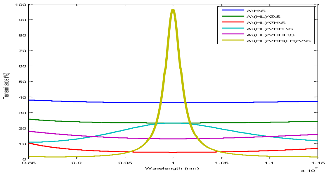
Figure(1) Transmittance as a function of wavelength for suggestion designs
