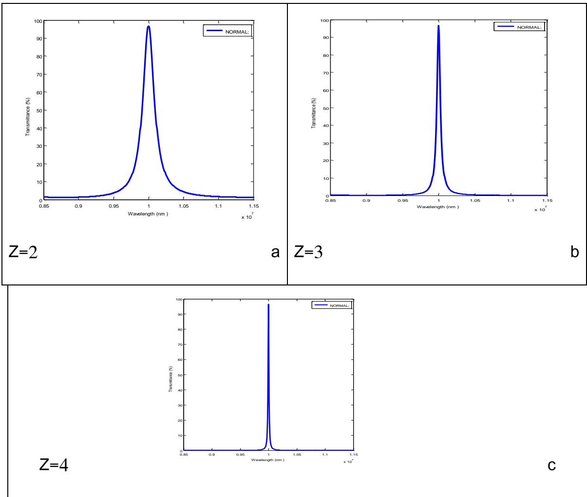
Figure(2) Transmittance as a function of wavelength at Z=2, Z=3, Z=4 At Normal Incident
