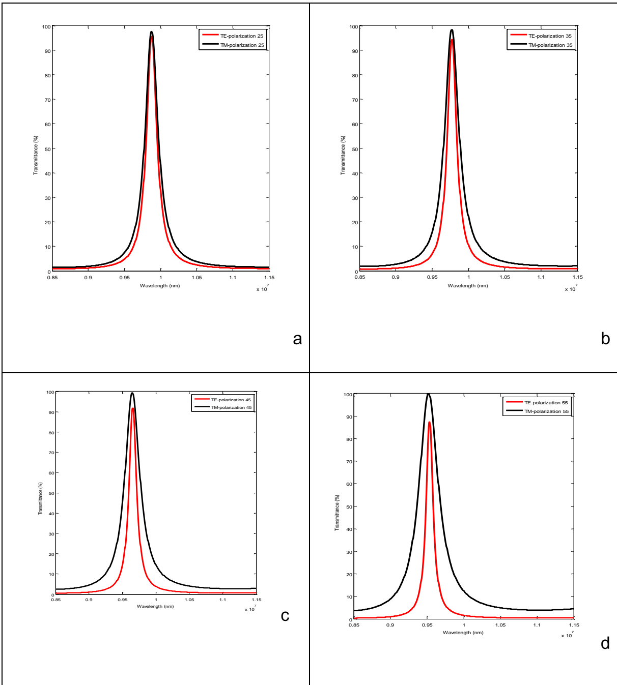
Transmittance as a function of wavelength at the Incident of angle (25°, 35°, 45°, 55°)
