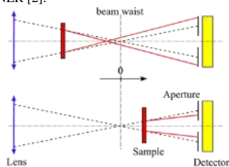
Fig .1: Z-scan process to vary the intensity of the laser beam, when the sample is moving along a focused beam. Laser intensity varied continuously with maximum at the focal point. Dashed line: laser beam transmission deprived of a sample. Solid line: intensive by a sample beam [2].
