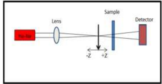
Fig.3: Experimental setup.
