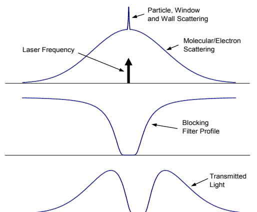
Fig. (4) Basic Filtered Rayleigh Scattering concept
