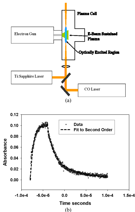
Fig. (1) Apparatus (a) and typical time dependent electron density trace (b) from O_2 free electron attachment mitigation studies of Frederickson
