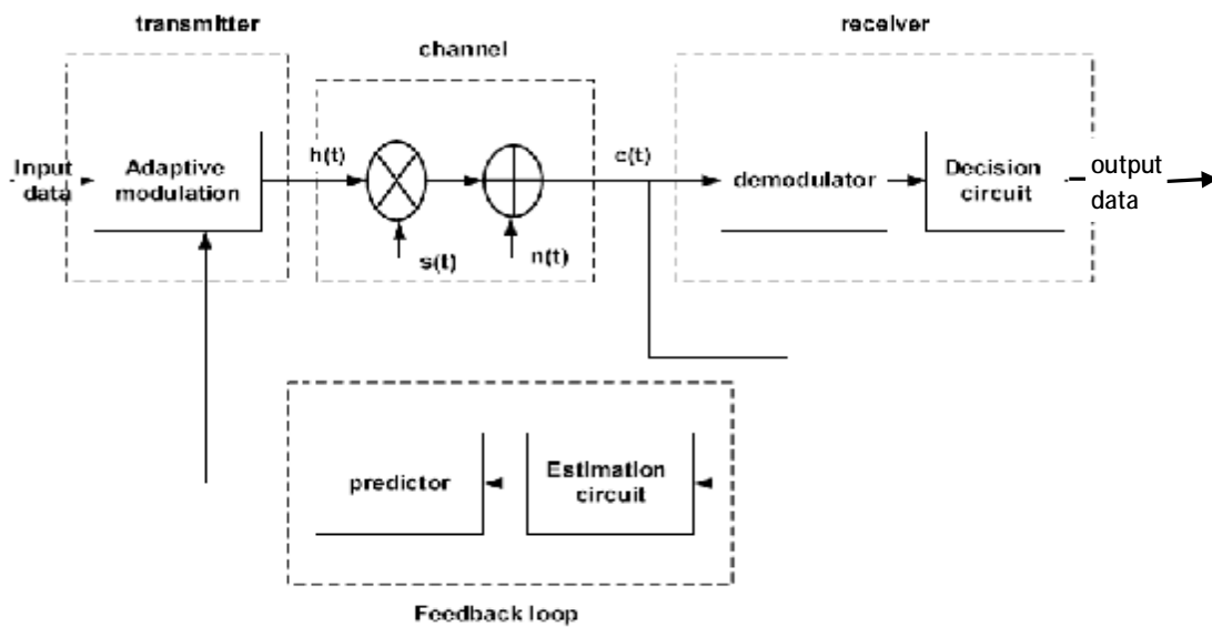
Figure (4) proposed system
