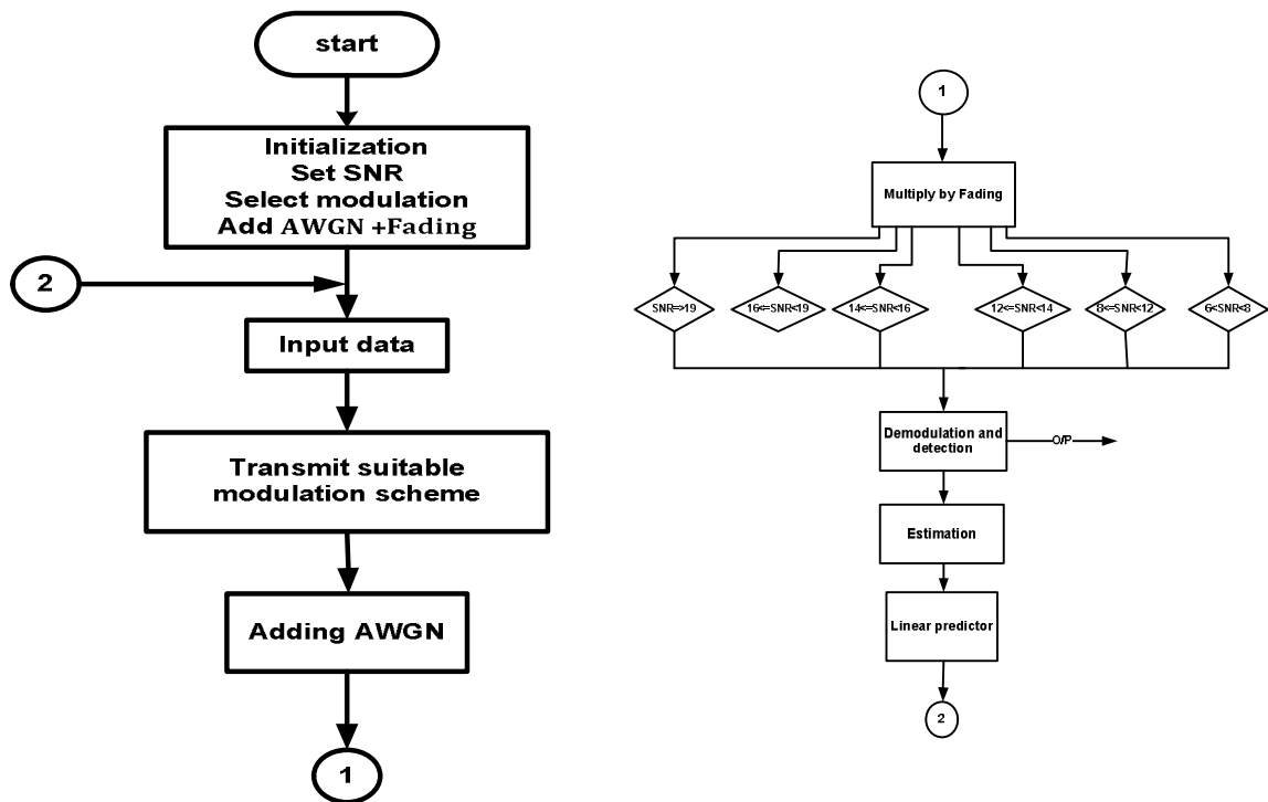
Figure (5) Flow chart of the designed system
