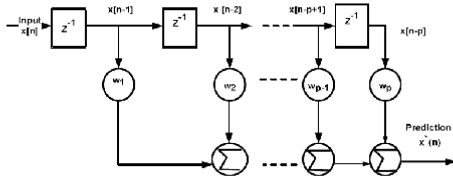
Figure (3) Block diagram of linear prediction filter of order p
