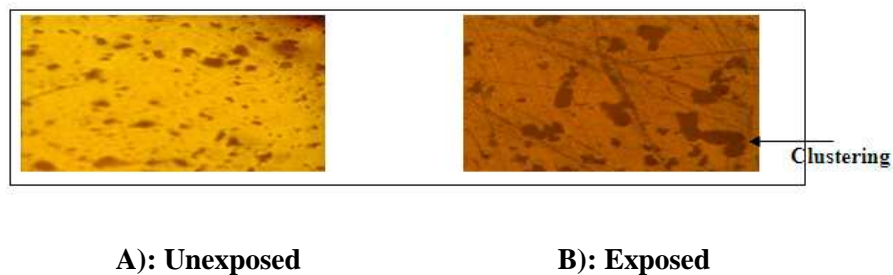
Figure (5): Optical micrographs of PMMA doped methyl orange at 6.7 \times 10^{-2} concentration samples A) unexposed, B) exposed to UV- irradiation (75x).
