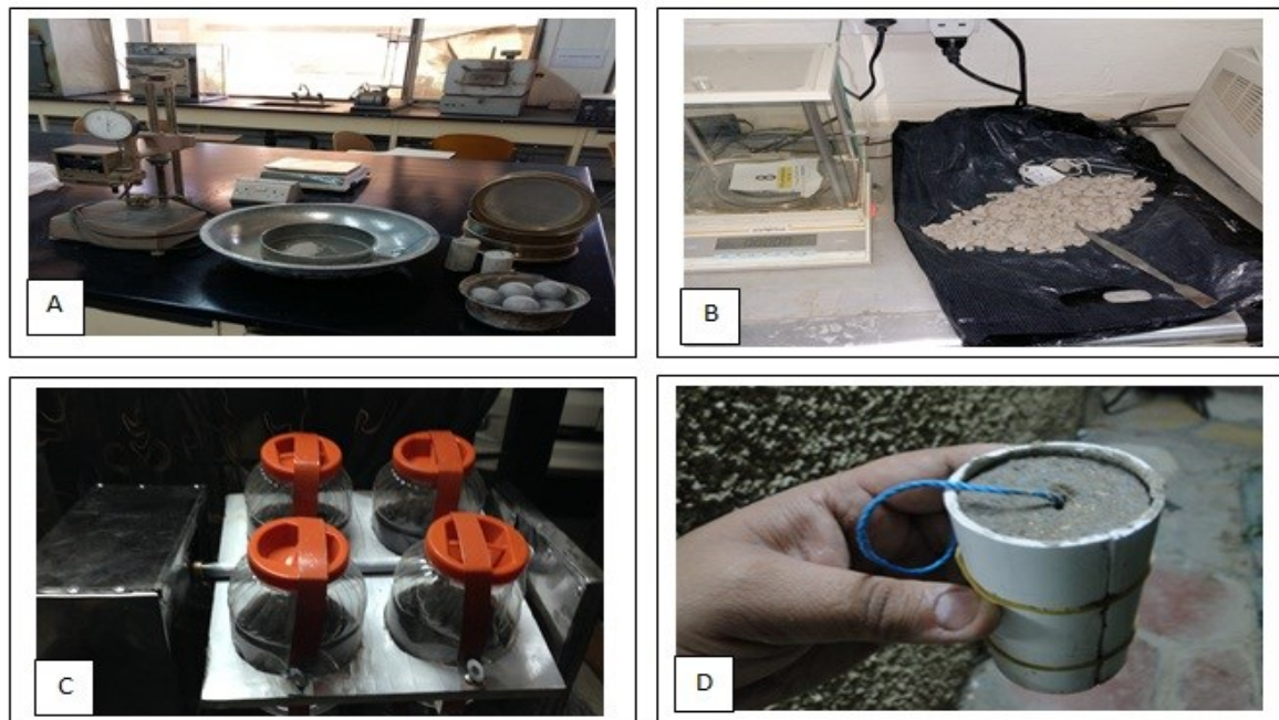
Figure 2: Experimental Procedure and apparatus, A) Specimen Preparation B) Crushing the Sample C) Agitation Process D) Sampling for Leaching Test
