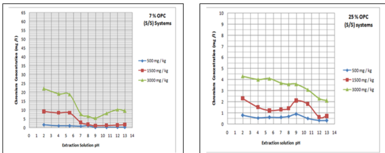
Figure 3: LSP As a function of pH chromium ions leaching from Cement-based S (S/S) samples.
