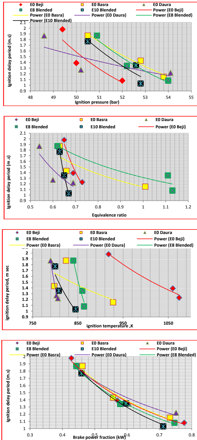
Figure (10): The ignition delay results obtained (a) ignition pressure (b) equivalence ratio, (c) ignition temperature, and (d) brake power fraction.
