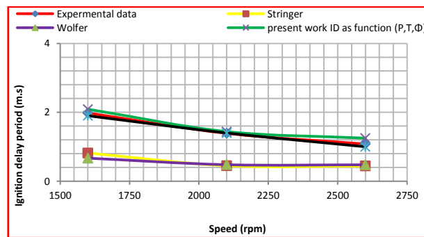
Figure (11): Variation of ignition delay for different ID empirical equations at all engine speeds using E0 Beji at 10N.m.
