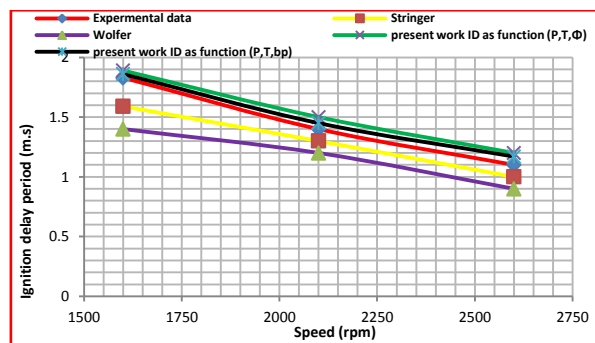
Figure (12): Variation of ignition delay for different empirical equations at all engine speeds using E0 Basra at 10N.m .
