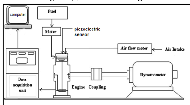
Figure (2): Schematic diagram of the test diesel engine.
