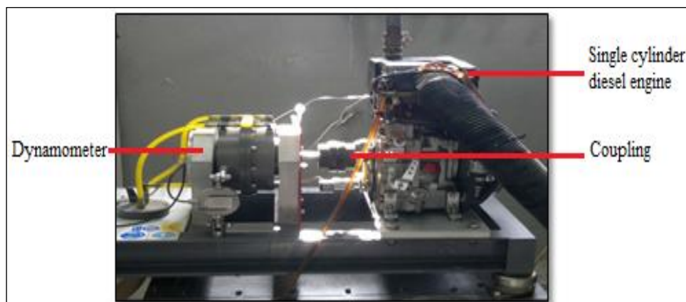
Figure (1): Test diesel engine.
