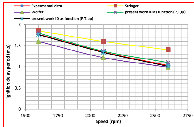
Figure (15): Variation of ignition delay for different ID empirical equations at all engine speeds using E10 Blended at 10N.m .
