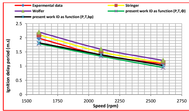
Figure (14): Variation of ignition delay for different ID empirical equations at all engine speeds using E8 Blended at 10N.m .
