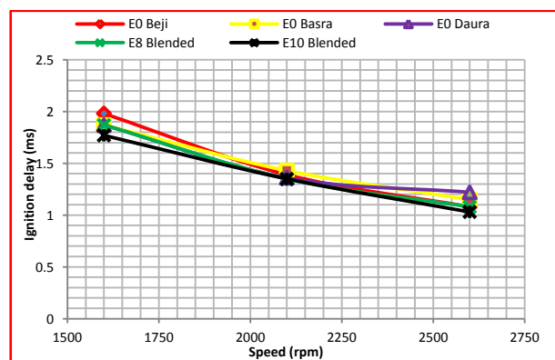
Figure (8): Effect of speed on the ignition delay for diesel fuels and ethanol- diesel blends.
