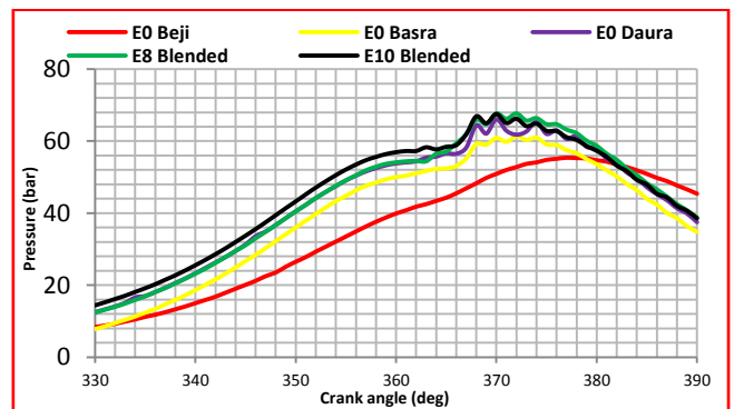
Figure (6): Measured pressure as a function of crank angle for diesel and ethanol-diesel blended at torque =10Nm at speed 2600rpm.
