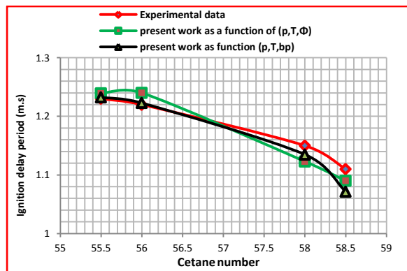
Figure (9): Effect of Cetane number on the ignition delay.
