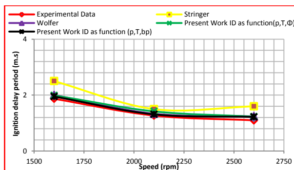
Figure (13): Variation of ignition delay for different ID empirical equations at all engine speeds using E0 Daura at 10N.m .
