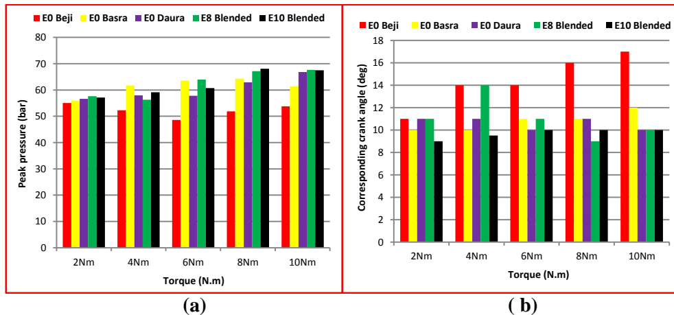
Figure (7): Effect of diesel and ethanol-diesel blended on (a) maximum combustion pressure and (b) its corresponding crank angle for varying torque at speed 2600 rpm
