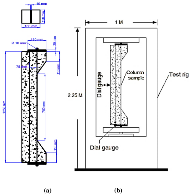
Figure 5. a) Eccentricity loading Setup, b) Installing measurements devices of column specimen
