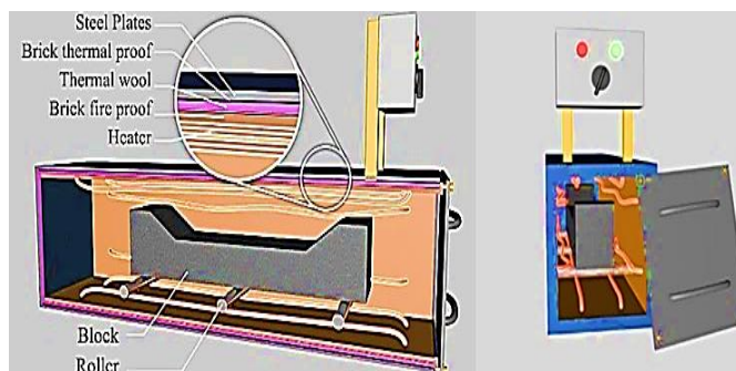
Figure 3. Close-up details of the electric furnace.
