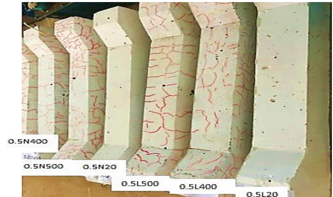
Figure 6. The thermal crack pattern for heated columns
