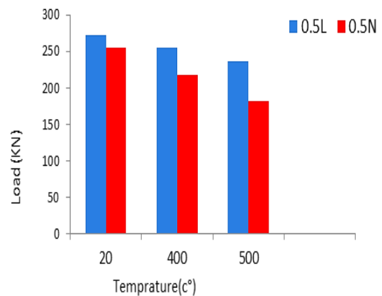
Figure 12. Effect of elevated temperature on ultimate load capacity of LWRC columns, and NWRC columns
