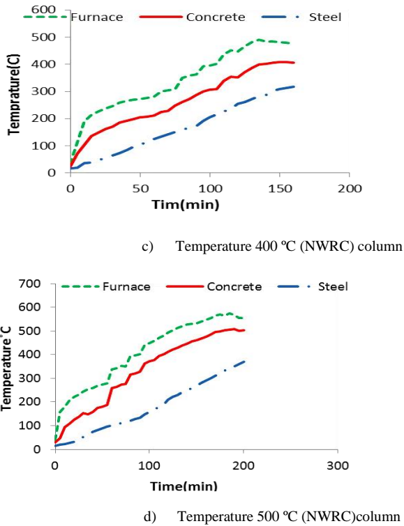
Figure 7. Time-temperature histories of LWRC columns and NWRC columns under different elevated temperature
