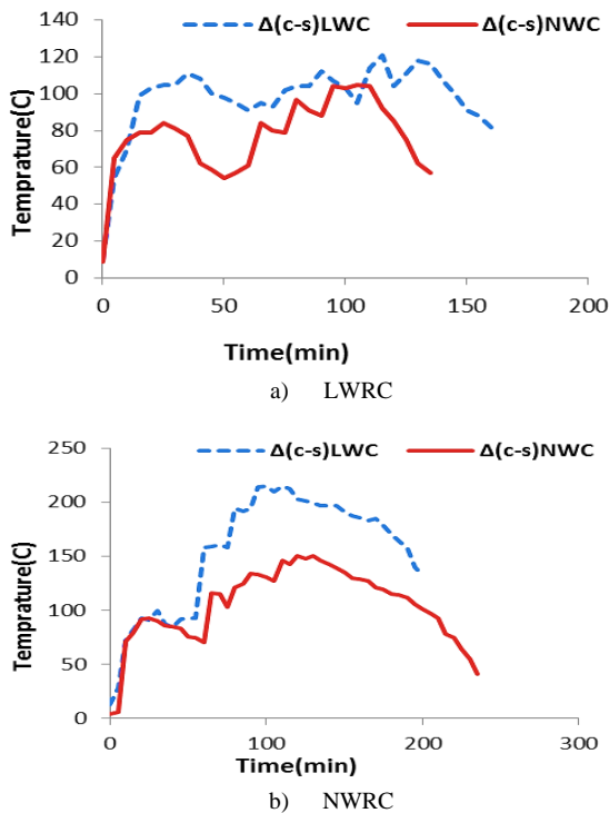
Figure 8. The difference between the temperature of concrete surface and steel bars surface with time for a) LWRC, b) NWRC columns under different elevated temperatures.
