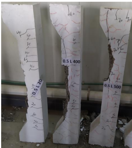
Figure 9. column specimen failure for 0.5L20, 0.5L400, 0.5L500
