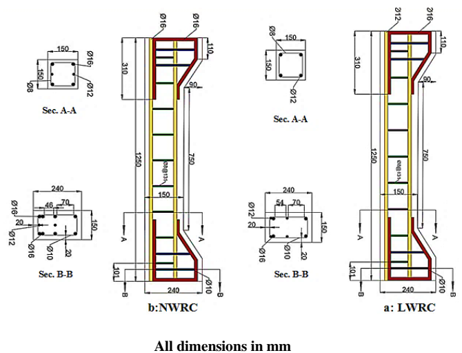
Figure 2. Dimensions and reinforcement details of RC column specimens
