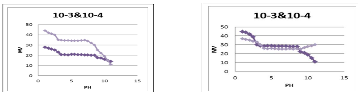
Figure (4): Typical plot of electrode response versus pH of DOMP-MIP electrodes at different Concentrations.
