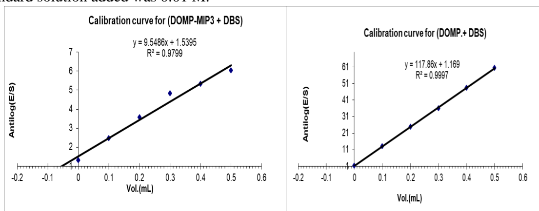
Figure (7): Variation of antilog (E/S) of synthetic solution of 1 \times 10^{-3} , 1 \times 10^{-4} M versus of standard DOMP added using electrode (IQ).
