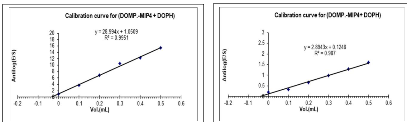
Figure (8): Variation of antilog (E/S) of synthetic solution of 1 \times 10^{-3} , 1 \times 10^{-4} M versus of standard DOMP added using electrode (IIIQ).
