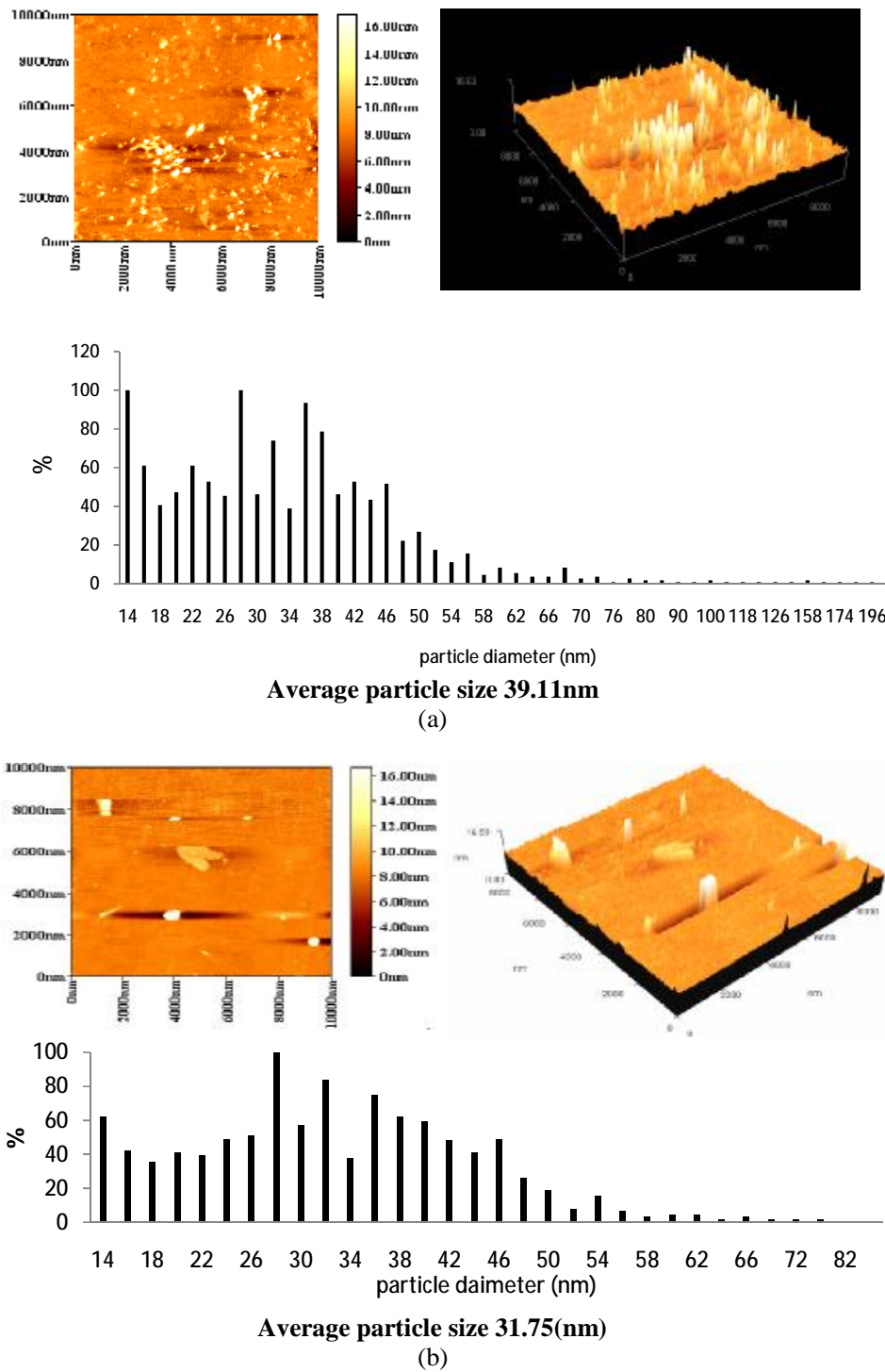
Figure (4) Surface morphology of ZnO NPs prepared at 1.06 mm laser wavelength 25 \text{ J/cm}^2 (a) at 20 laser pulses (b) at 60 laser pulses.
