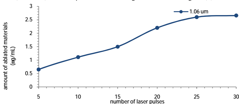
Figure (2) Amount of ablated materials as a function of number of pulses for 1.064 \mu\text{m} laser wavelength at 25 J/cm 2 laser fluence.
