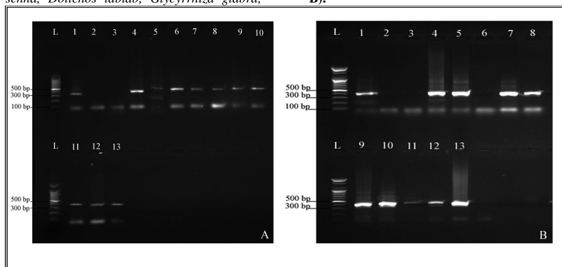
Figure 1. Gel electrophoresis of PCR products from 13 samples of DNA amplified using primers. (A) represented primer ITS5/P2 for ITS-1 region and (B) represented primer ITS3/ITS4 for ITS-2 region. Lane L molecular size marker one step 100 bp ladder (Promega). Lane 1-13 species under study (1- Albizia julibrissin 2- Alhagi camelorum 3- Bauhinia alba 4- Caesalpinia gilliesii 5- Cassia didymobotrya 6- Cassia senna 7- Dolichos lablab 8- Glycyrrhiza glabra 9- Medicago sativa 10- Melilotus officinalis 11- Trifolium purpureum 12- Trigonella foenum-graecum 13- Vicia faba )
