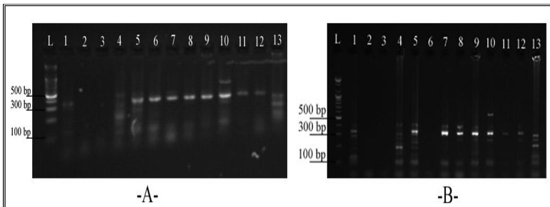
Figure 2. Restriction digestion patterns obtained after electrophoresis on a 2% agarose gel of 13 samples of DNA amplified using primers and digested with CfoI . (A) represented primer ITS5/P2 for ITS-1 region and (B) represented primer ITS3/ITS4 for ITS-2 region. Lane L molecular size marker one step 100 bp ladder (Promega), Lane 1-13 species under study (1- Albizia julibrissin 2- Alhagi camelorum 3- Bauhinia alba 4- Caesalpinia gilliesii 5- Cassia didymobotrya 6- Cassia senna 7- Dolichos lablab 8- Glycyrrhiza glabra 9- Medicago sativa 10- Melilotus officinalis 11- Trifolium purpureum 12- Trigonella foenum-graecum 13- Vicia faba
