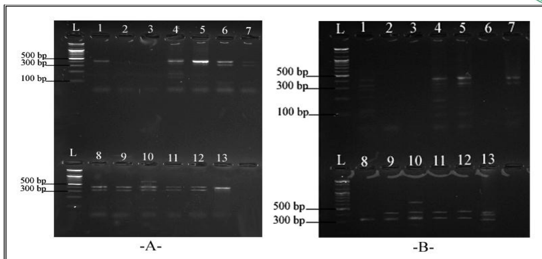
Figure 3. Restriction digestion patterns obtained after electrophoresis on a 2% agarose gel of 13 samples of DNA amplified using primers and digested with Hha I. (A) represented primer ITS5/P2 for ITS-1 region and (B) represented primer ITS3/ITS4 for ITS-2 region. Lane L molecular size marker one step 100 bp ladder (Promega). Lane 1-13 species under study (1- Albizia julibrissin 2- Alhagi camelorum 3- Bauhinia alba 4- Caesalpinia gilliesii 5- Cassia didymobotrya 6- Cassia senna 7- Dolichos lablab 8- Glycyrrhiza glabra 9- Medicago sativa 10- Melilotus officinalis 11- Trifolium purpureum 12- Trigonella foenum-graecum 13- Vicia faba
