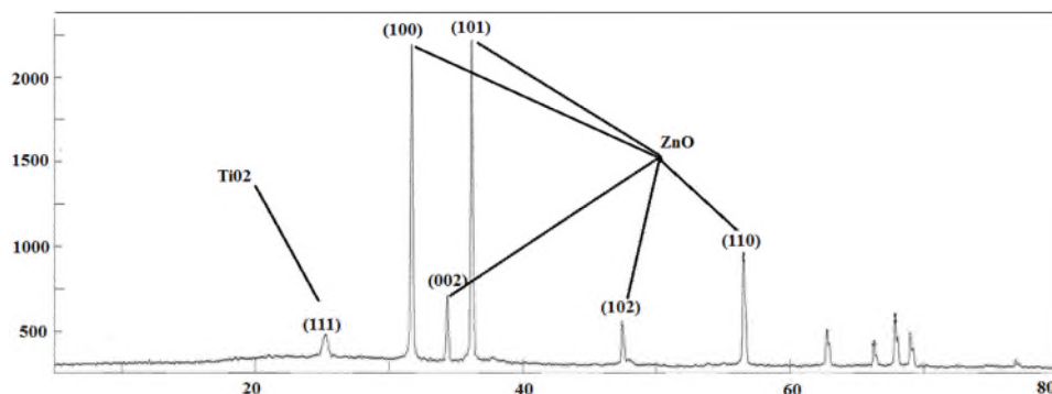
Figure (1) XRD pattern for ZnO-TiO 2 thick film.
