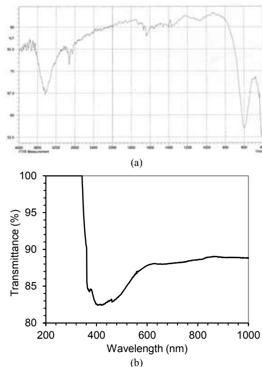
Fig. (2) The transmission FTIR (a) and UV-visible (b) spectra of the prepared sample
