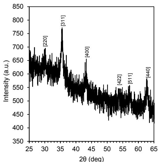
Fig. (3) The XRD pattern of the prepared sample
