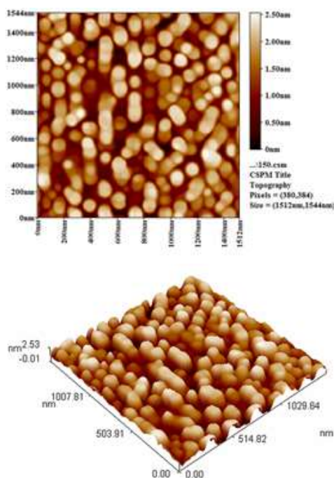
Fig. (5) The AFM image of the prepared sample
