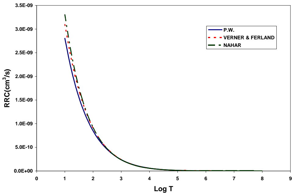
FIG.(6):Radiative recombination rate coefficient for Na IX-ion compared with VERNER & FERLAND (1996) and NAHAR (2006) calculations.
