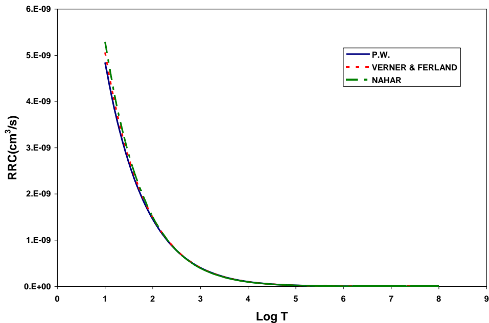
FIG.(13):Radiative recombination rate coefficient for Mg xi-ion compared with VERNER & FERLAND (1996) and NAHAR (2006) calculations.
