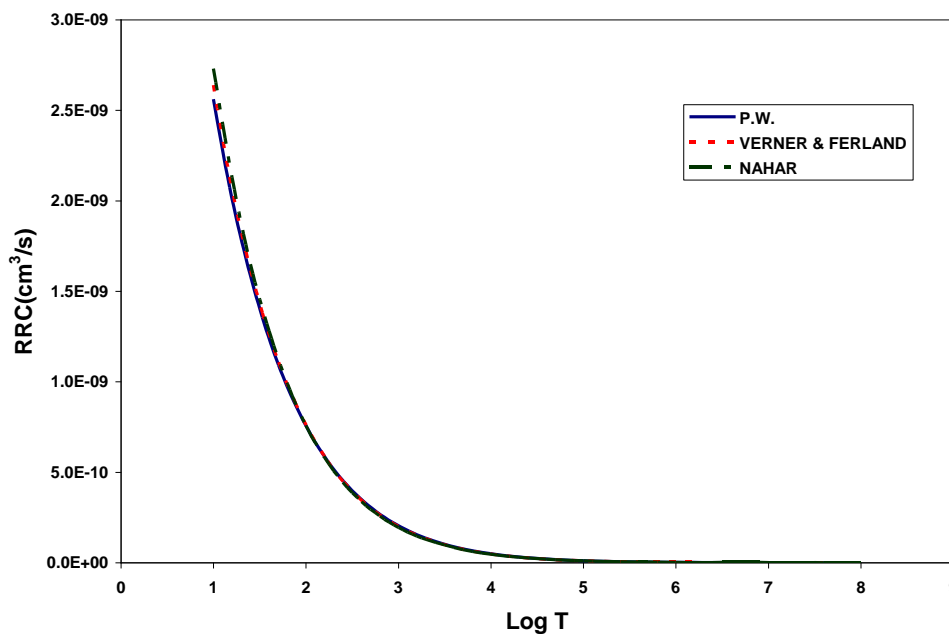
FIG.(3):Radiative recombination rate coefficient for F VIII-ion compared with VERNER & FERLAND (1996) and NAHAR (2006) calculations.
