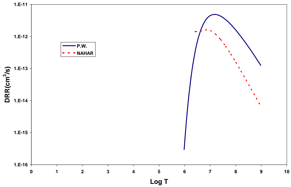
FIG.(22):The dielectronic recombination rate coefficient for Mg x-ion compared with NAHAR (2006) data
