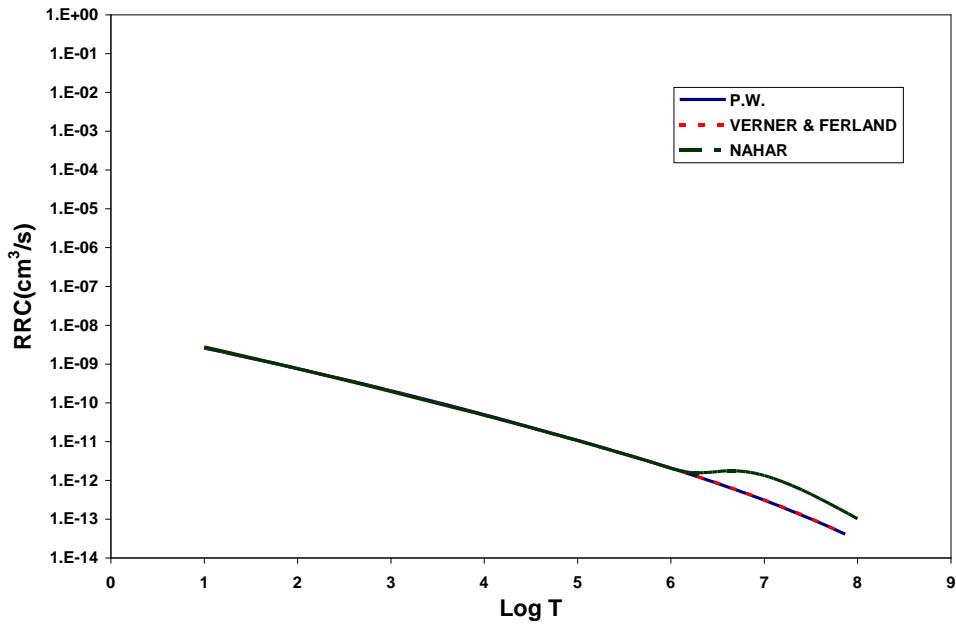
FIG.(4):The same for FIG.(3) in logarithmic scale for RRC to see the dielectronic effects arise for NAHAR at LogT>6.2
