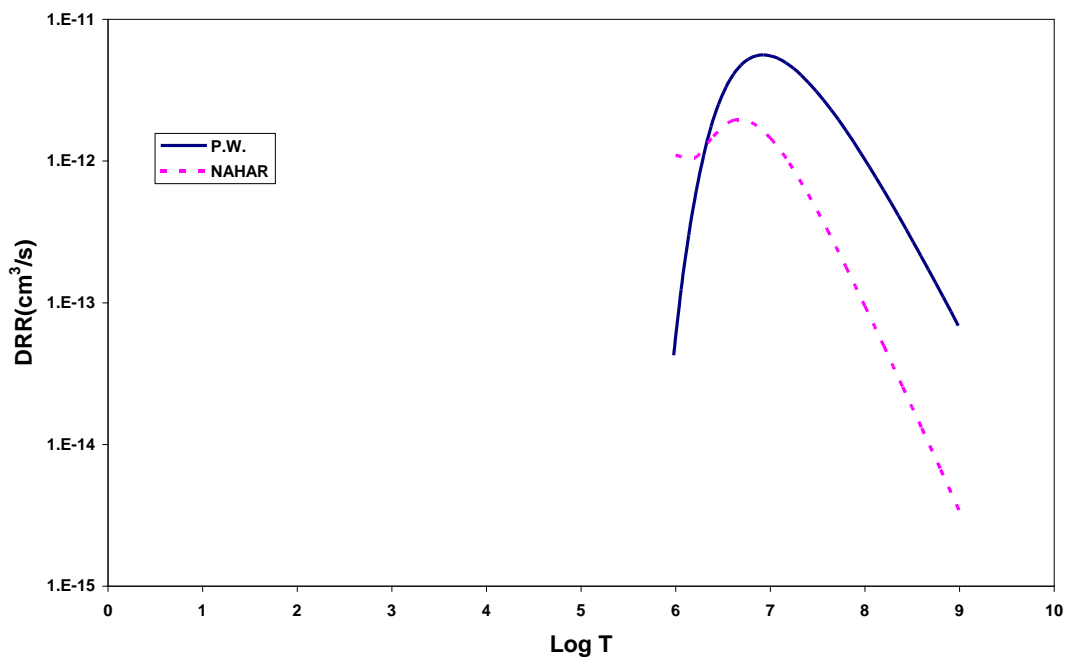
FIG.(20):The dielectronic recombination rate coefficient for F VII-ion compared with NAHAR (2006) data.
