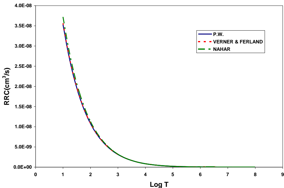
FIG.(18):Radiative recombination rate coefficient for Ni xxviii-ion compared with VERNER & FERLAND and NAHAR calculations.
