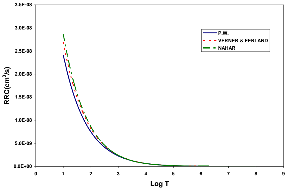
FIG.(16):Radiative recombination rate coefficient for Ni XXVI-ion compared with VERNER & FERLAND (1996) and NAHAR (2005) calculations.
