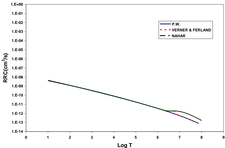
FIG.(9):The same for FIG.(8) in logarithmic scale for RRC to see the dielectric effects arise for NAHAR at LogT>6.4
