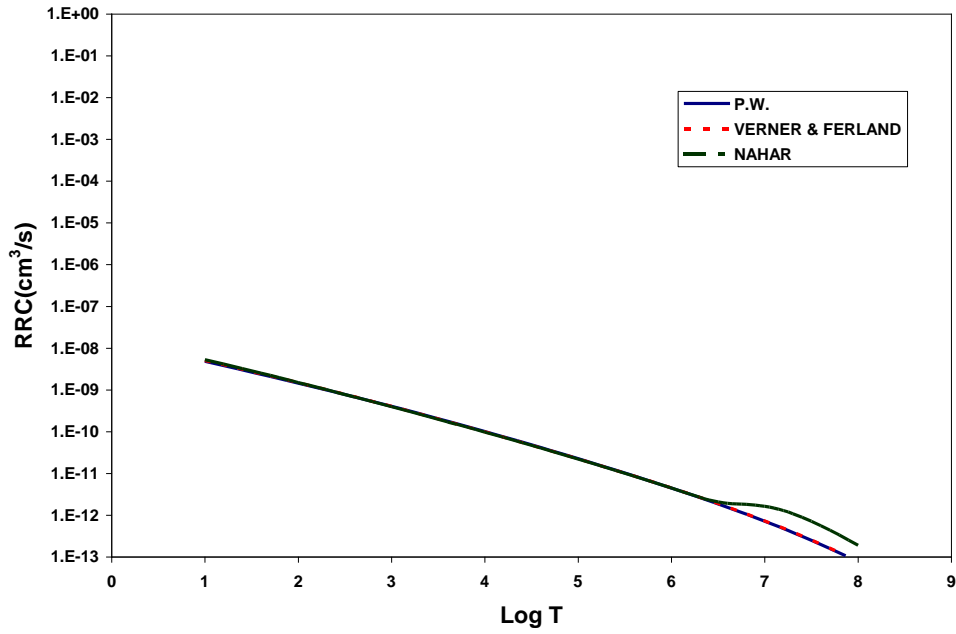
FIG.(14):The same for FIG.(13) in logarithmic scale for RRC to see the dielectronic effects arise for NAHAR at LogT>6.6
