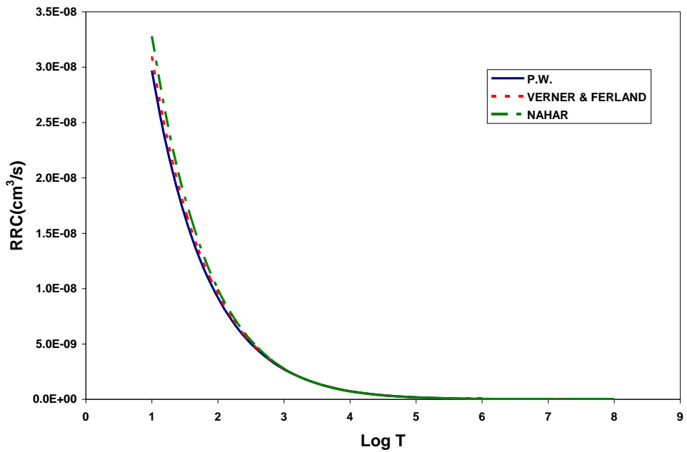
FIG.(17):Radiative recombination rate coefficient for Ni XXVII-ion compared with VERNER & FERLAND (1996) and NAHAR (2005) calculations.
