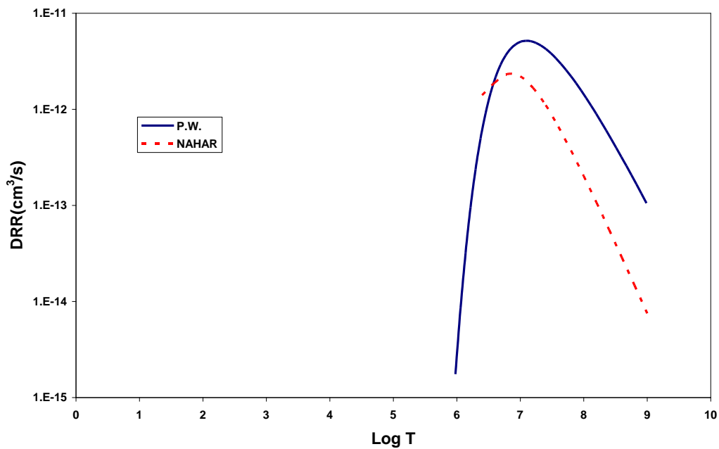
FIG.(21):The dielectronic recombination rate coefficient for Na IX-ion compared with NAHAR (2006) data
