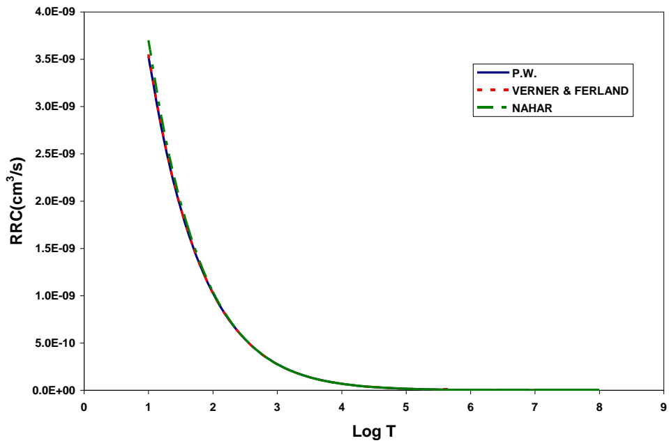
FIG.(5):Radiative recombination rate coefficient for F IX-ion compared with VERNER & FERLAND (1996) and NAHAR (2006) calculations.
