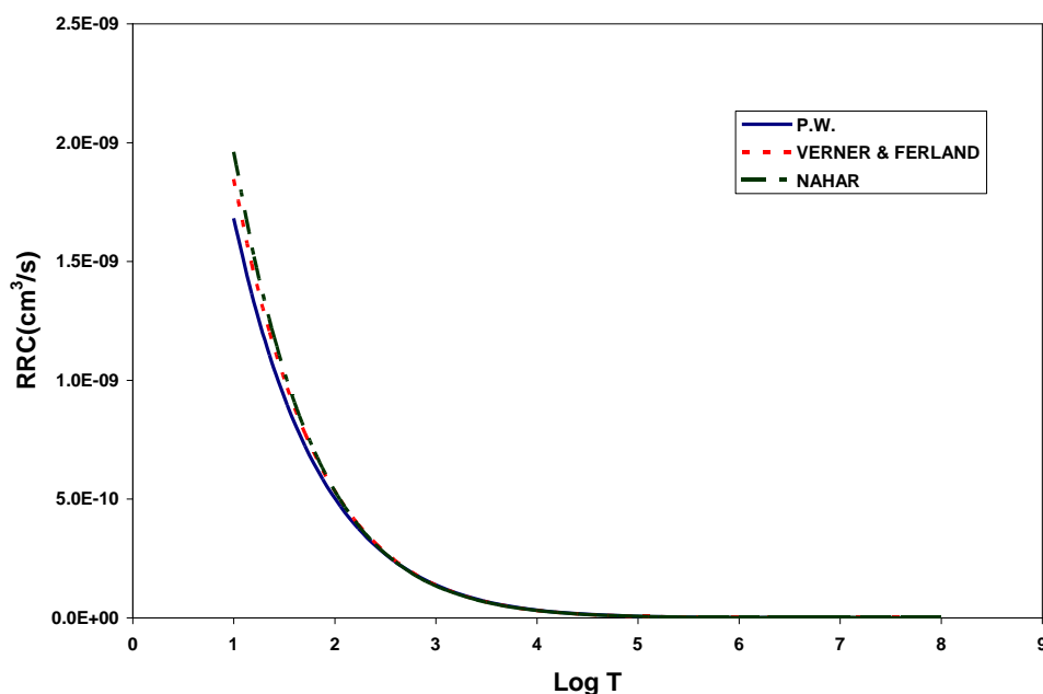
FIG.(1): Radiative recombination rate coefficient for F VII-ION compared with VERNER & FERLAND (1996) and NAHAR (2006) calculations.
