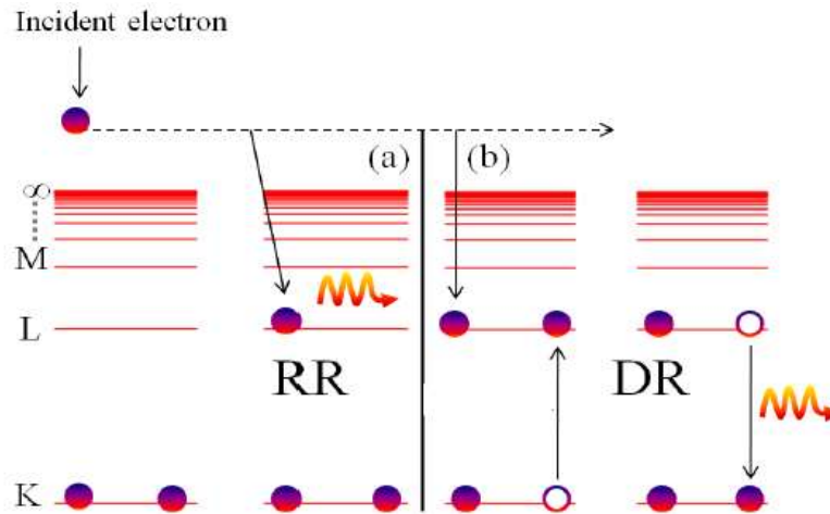
Figure(1): Schematic diagram [1] of: (a) Radiative recombination (b) Dielectronic recombination in He-like ion
