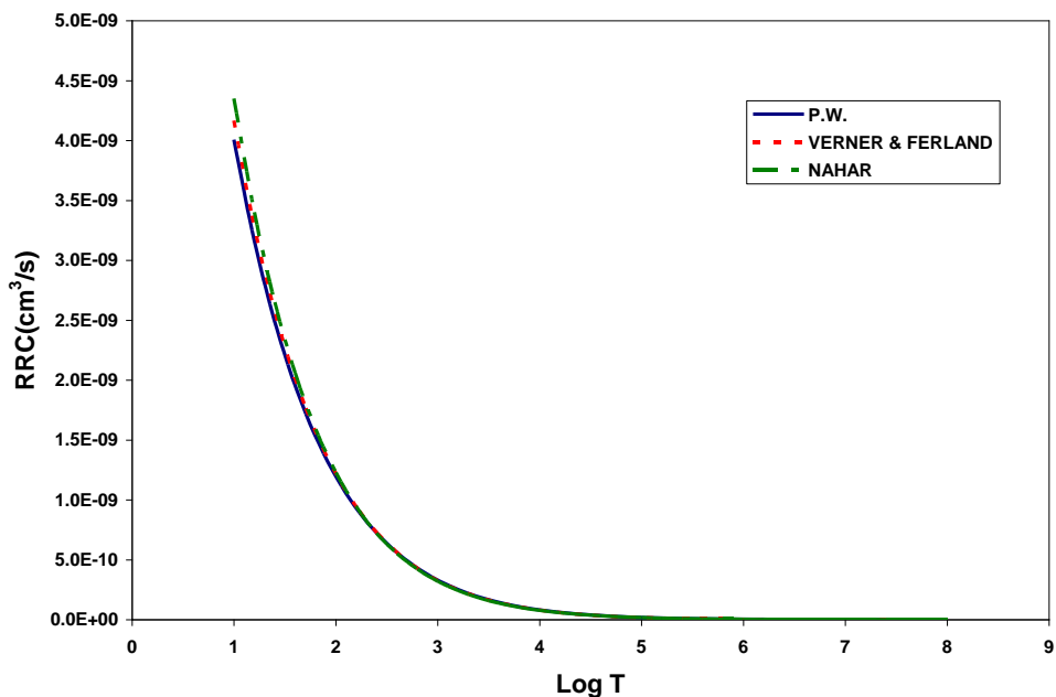
FIG.(8):Radiative recombination rate coefficient for Na x-ion compared with VERNER & FERLAND (1996) and NAHAR (2006) calculations.
