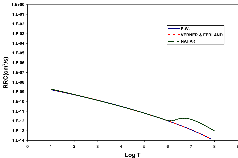
FIG.(2):The same for FIG.(1) in logarithmic scale for RRC to see the dielectronic effects arise for NAHAR at LogT>6.
