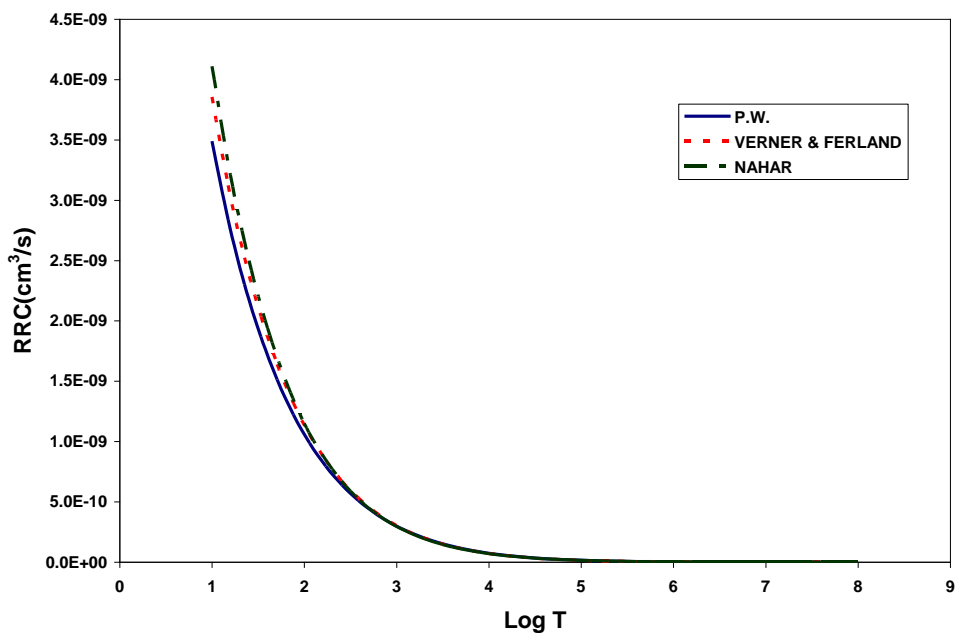
FIG.(11):Radiative recombination rate coefficient for Mg x-ion compared with VERNER & FERLAND (1996) and NAHAR (2006) calculations.
