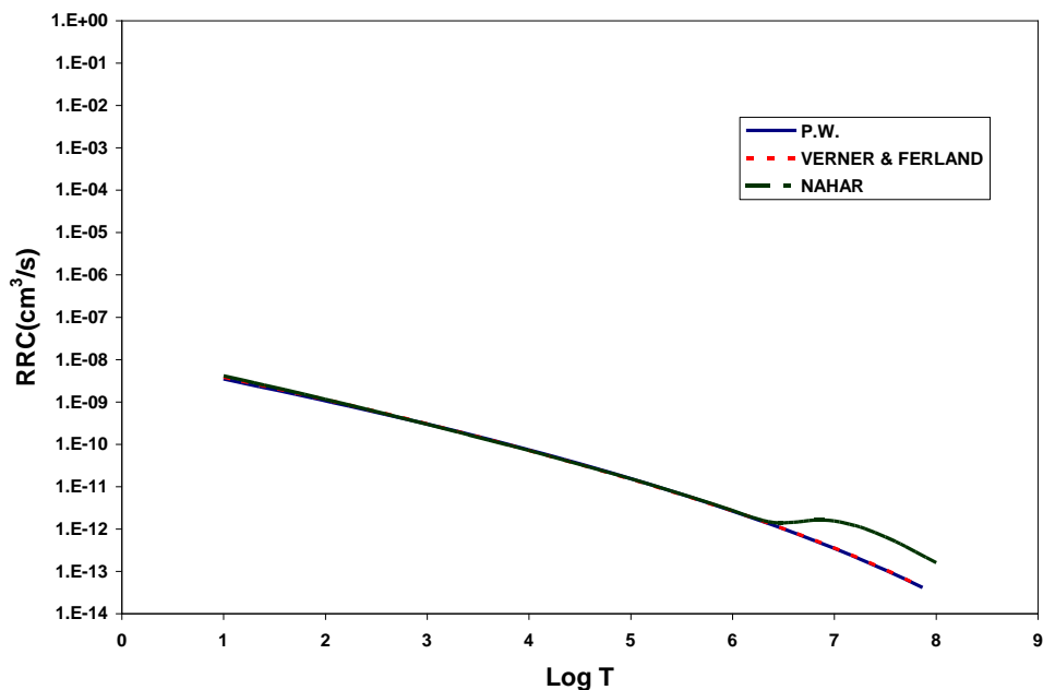
FIG.(12):The same for FIG.(11) in logarithmic scale for RRC to see the dielectronic effects arise for NAHAR at LogT>6.4
