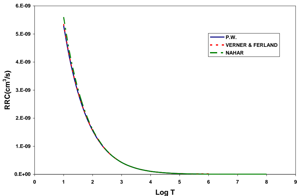
FIG.(10):Radiative recombination rate coefficient for Na XI-ion compared with VERNER & FERLAND (1996) and NAHAR(2006) calculations.
