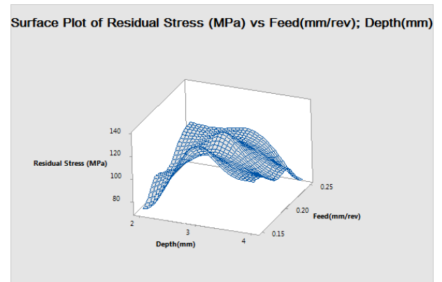
Figure 6: Relationship between residual stress and process parameters.
