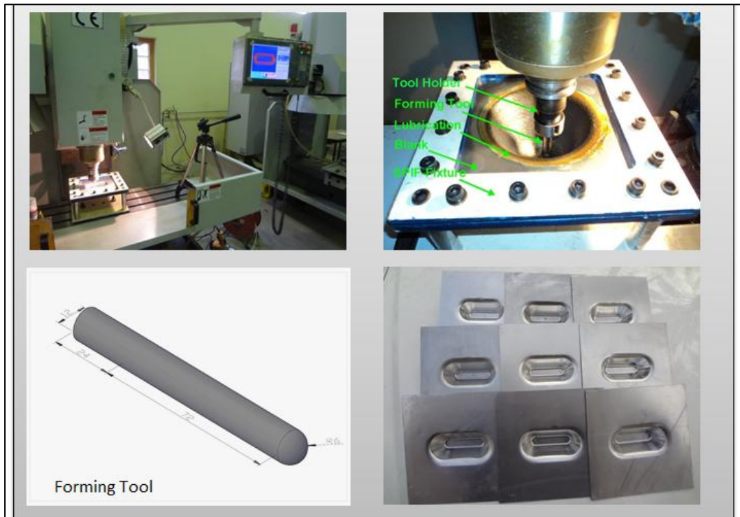
Figure 3: The experimental setup and nine-samples
