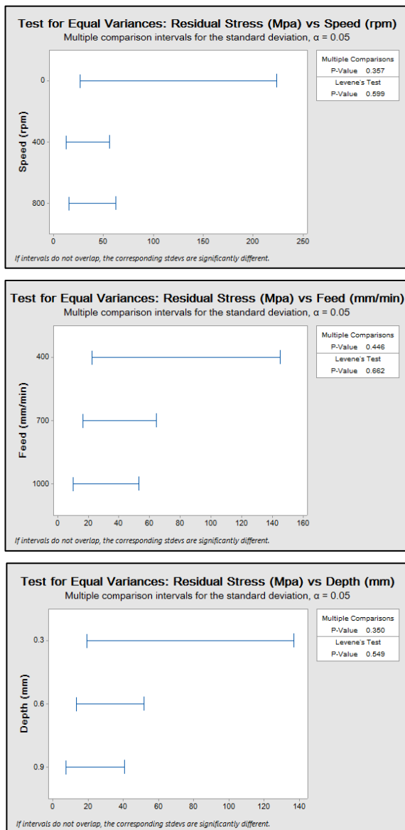
Figure 9: Variance of residual stress with respect to process parameters
