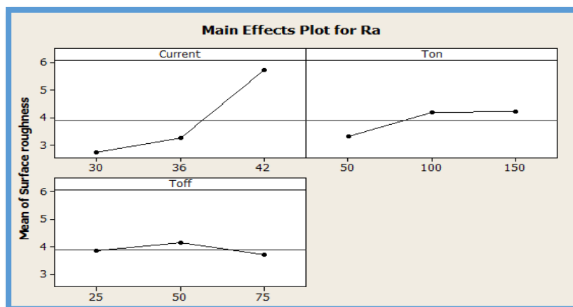
Figure 10: Mean effects plot for Surface roughness
