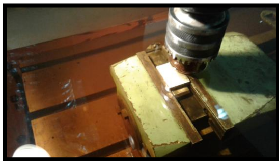
Figure 2: Work-Holding Assembly
