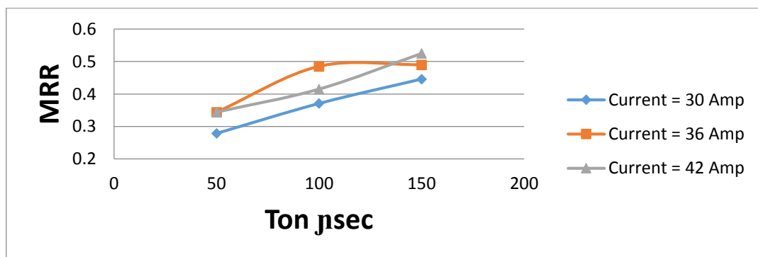
Figure 7: Effect of Pulse on Time and current on the MRR
