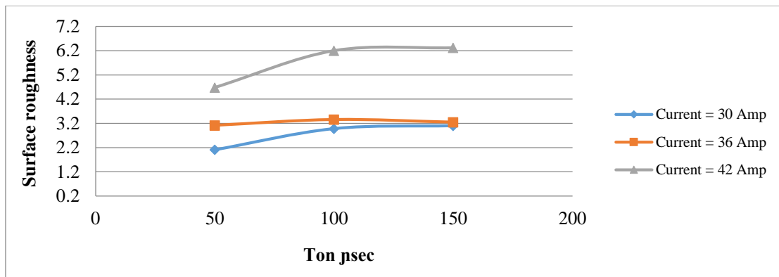
Figure 9: Effect of Pulse on Time and current on the Surface roughness
