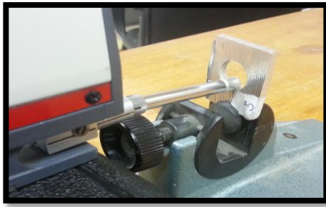
Figure 6: Pocket Surf holder for the proposed work
