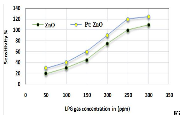
Figure 11: Sensitivity curve of the sensor with LPG gas concentration.
