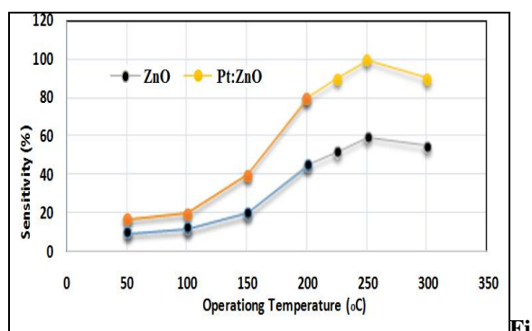
Figure 12: Sensitivity versus operating temperature at 250 ppm LPG
