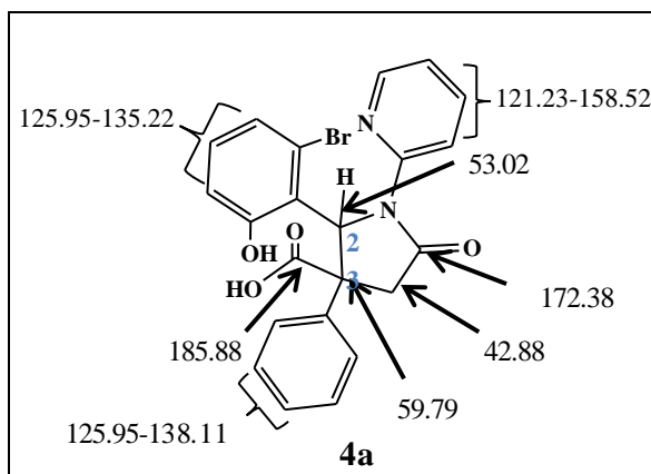
Figure 15: 13 C-NMR spectrum of 4a
