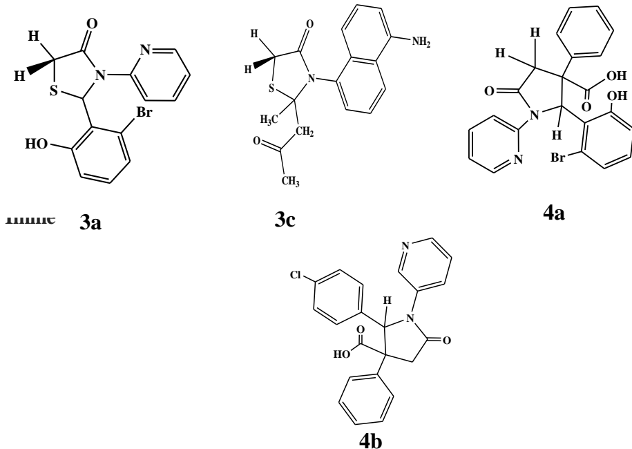
Figure 4 : prepared compounds
