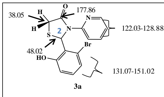
Figure 13 : 13 C-NMR spectrum of 3a
