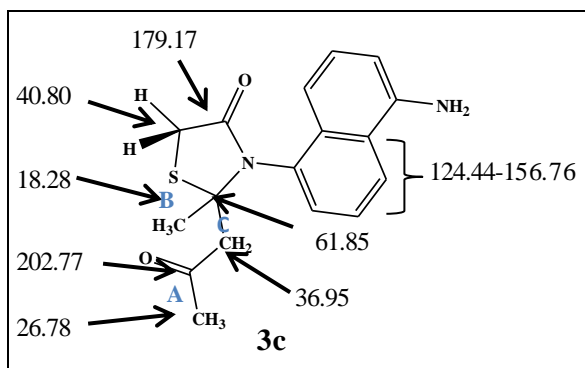
Figure 14 : 13 C-NMR spectrum of 3c
