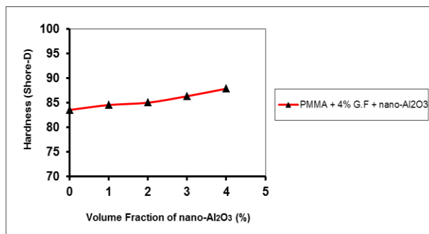
Figure 13: Hardness of PMMA Hybrid Laminated Composite as Function of (Nano- \text{Al}_2\text{O}_3 ) Particles (Vol. %) in Composite.
