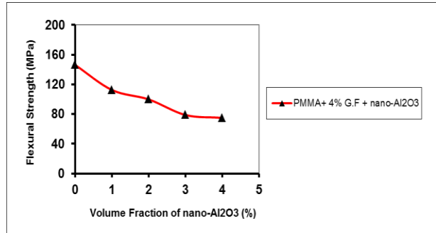
Figure 10: Flexural Strength of PMMA Hybrid Laminated Composite as Function of (Nano-Al 2 O 3 ) Particles (Vol. %) in Composite.
