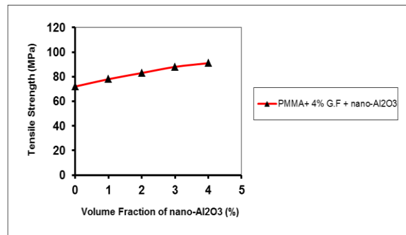
Figure 6: Tensile Strength of PMMA Hybrid Laminated Composite as Function of (Nano-Al 2 O 3 ) Particles (Vol. %) in Composite.
