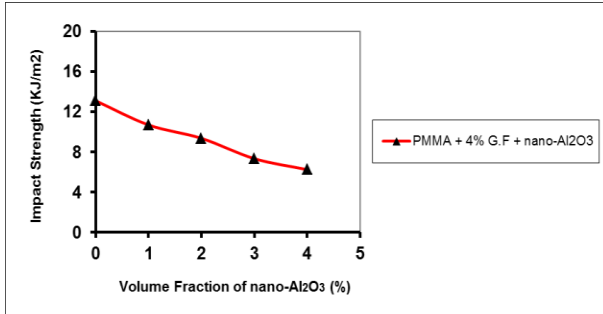
Figure 8: Impact Strength of PMMA Hybrid Laminated Composite as Function of (Nano-Al 2 O 3 ) Particles (Vol. %) in Composite.
