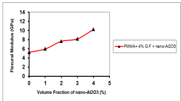
Figure 11: Flexural Modulus of PMMA Hybrid Laminated Composite as Function of (Nano-Al 2 O 3 ) Particles (Vol. %) in Composite.
