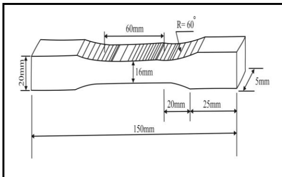
Figure 5: Schematic Specimen for Standard Specimen of Tensile Test.
