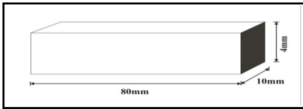
Figure 7: Schematic Specimen for Standard Specimen of Impact Test.
