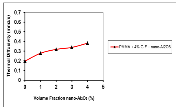
Figure 17: Thermal Diffusivity of PMMA Hybrid Laminated Composite as Function of (Nano-Al 2 O 3 ) Particles (Vol. %) in Composite.
