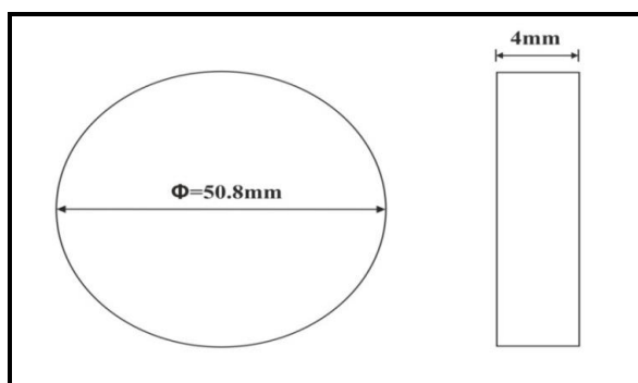
Figure 12: Schematic Specimen for Standard Specimen of Hardness Test.
