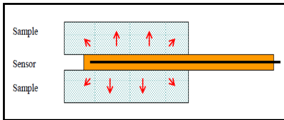
Figure 15: Hot Disk Sensor Operation.
