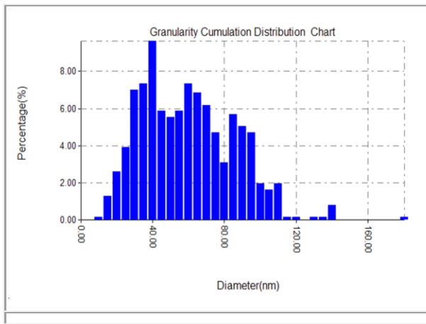
Figure 2: AFM Test of Nano-Al 2 O 3 Particles.
