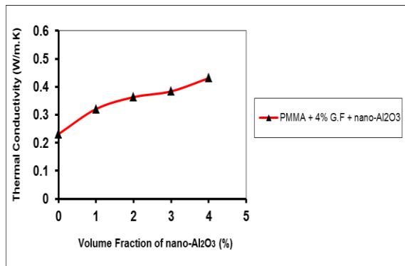
Figure 16: Thermal Conductivity of PMMA Hybrid Laminated Composite as Function of (Nano-Al 2 O 3 ) Particles (Vol. %) in Composite.
