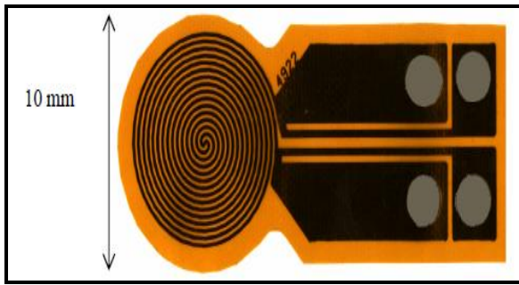
Figure 14: Hot Disk Sensor
