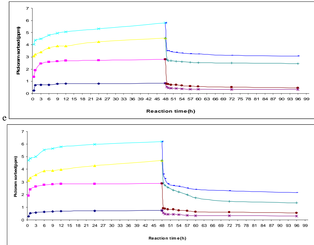
f- Fig. 1: Amount of picloram adsorbed-desorbed kinetically with time on selected soil samples (a) S 1 , (b) S 2 , (c) S 3 , (d) S 4 , (e) S 5 and (f) S 6 , (♦ 2, ■ 5, ▲ 10, and x 15 µgml -1 ).
