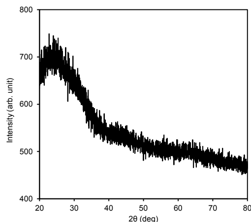
Fig. (2) XRD pattern of the optimum silicon dioxide sample prepared in this work
