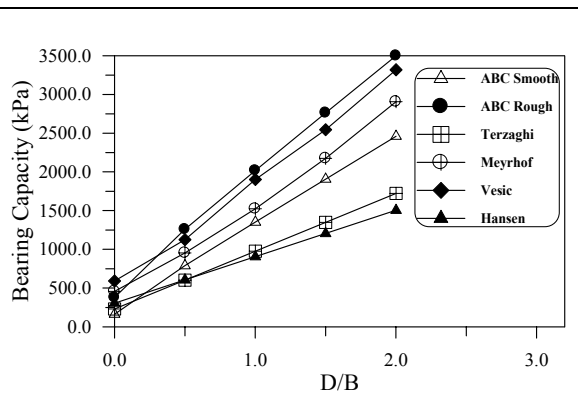
Fig. (13) – Bearing capacity for circular footing in sand ( \phi = 35^\circ ).
