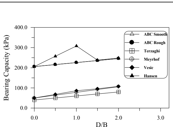
Fig. (15) – Bearing capacity for strip footing in clay ( c = 40 kPa).
