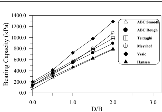
Fig. (19) – Bearing capacity for strip footing in sand ( \phi = 30^\circ ).
