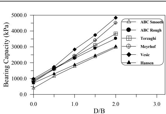
Fig. (21) – Bearing capacity for trip footing in sand ( \phi = 40^\circ ).
