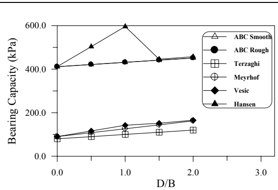
Fig. (17) – Bearing capacity for strip footing in clay ( c = 80 kPa).
