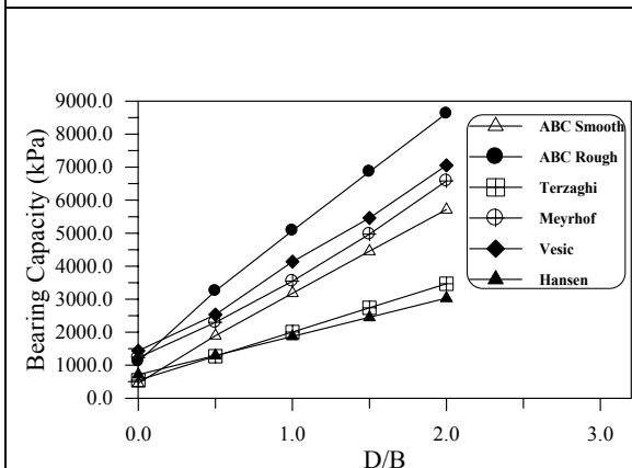
Fig. (14) – Bearing capacity for circular footing in sand ( \phi = 40^\circ ).
