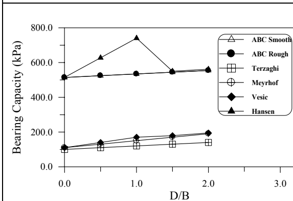
Fig. (18) – Bearing capacity for strip footing in clay ( c = 100 kPa).
