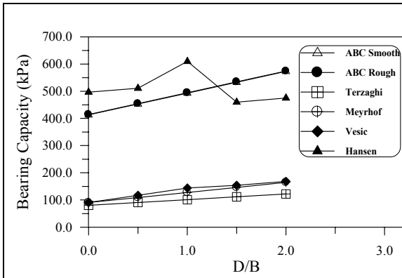
Fig. (28) – Bearing capacity for strip footing in clay (c = 80 kPa at surface).
