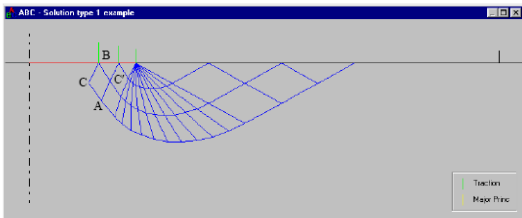
(e) CalcAB
