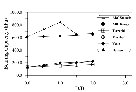
Fig. (11) – Bearing capacity for circular footing in clay ( c = 100 kPa).
