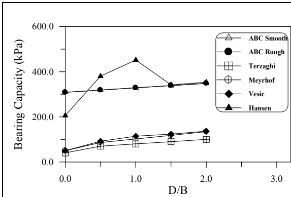
Fig. (16) – Bearing capacity for strip footing in clay ( c = 60 kPa).
