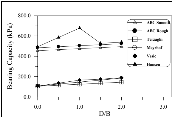
Fig. (10) – Bearing capacity for circular footing in clay ( c = 80 kPa).
