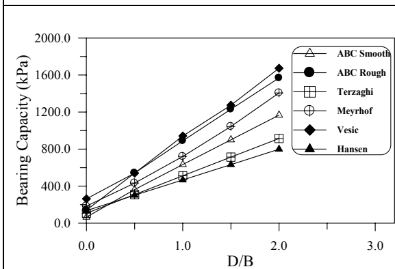
Fig. (12) – Bearing capacity for circular footing in sand ( \phi = 30^\circ ).
