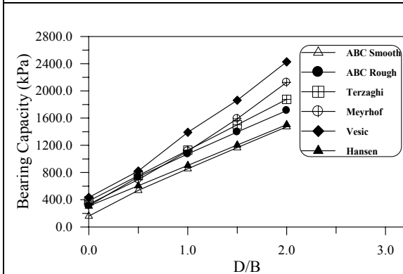
Fig. (20) – Bearing capacity for trip footing in sand ( \phi = 35^\circ ).
