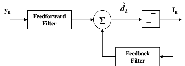
Figure (5) A decision-feedback equalizer
