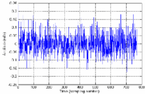
Figure (8) Wave form for OFDM signal in time domain
