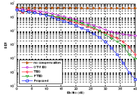
Figure (13) Performance of each equalizer in the OFDM system with insufficient cyclic prefix using case (B-2).
