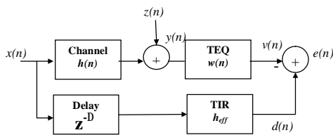
Figure (2) Structure of MMSE equalizer
