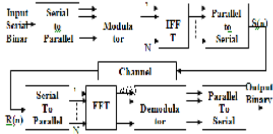
Figure (1) Block Diagram of the OFDM System
