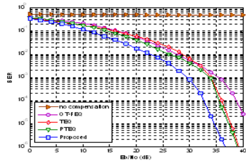
Figure (12) Performance of each equalizer in the OFDM system with sufficient cyclic prefix using case (B-1).
