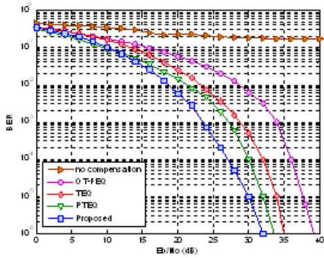
Figure (10) Performance of each equalizer in the OFDM system with sufficient cyclic prefix using case (A-1).
