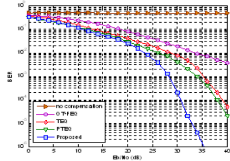
Figure (11) Performance of each equalizer in the OFDM system with insufficient cyclic prefix using case (A-2).
