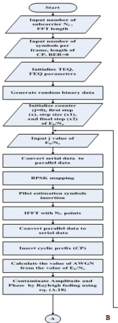
Figure (7) A flowchart of the proposed equalizer continued.....
