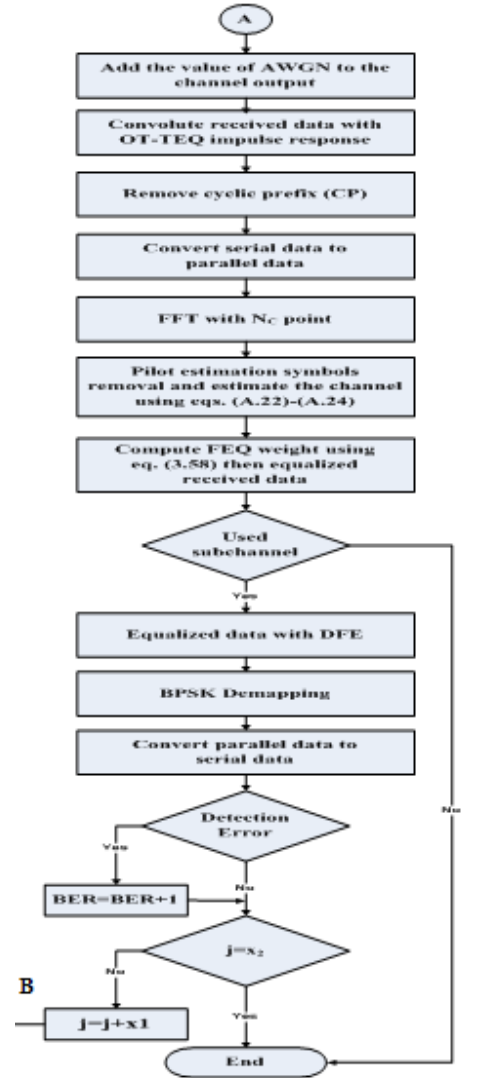
Figure (7)A flowchart of the proposed equalizer
