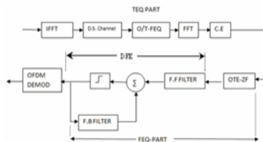
Figure (6) The proposed hybrid equalizer Structure
