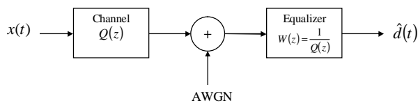
Figure (3) A simplified OFDM system
