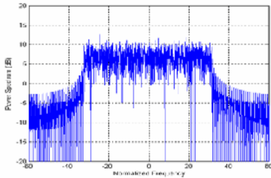
Figure (9) Spectrum of the OFDM signal
