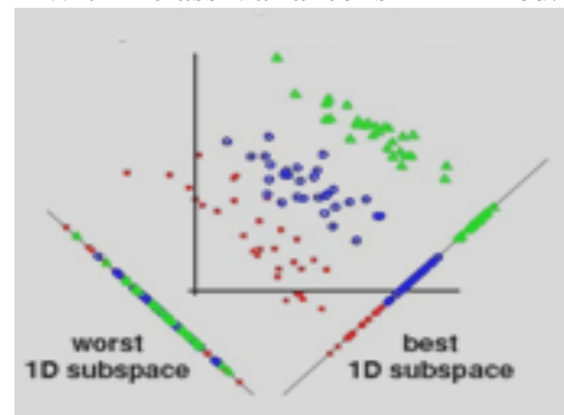
Fig(1): class feature data.
