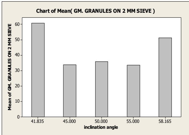
Fig. 3 The percentage 2mm granulated with respect to angle of inclination to IDG.
