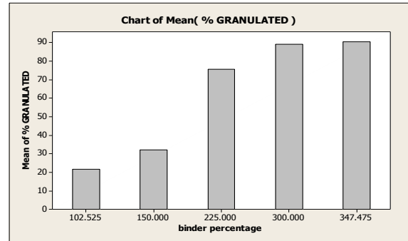
Fig. 14 The relationship of binder percentage to get the maximum total granules in RD Granulator
