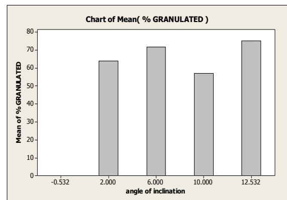
Fig.11 The relationship of angle of inclination to total granulation in the RD.
