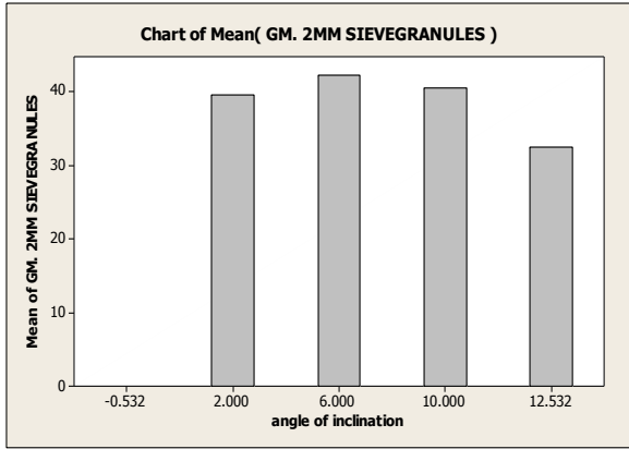
Fig. 12 The relationship of angle of inclination to get the maximum 2mm granules in RD Granulator
