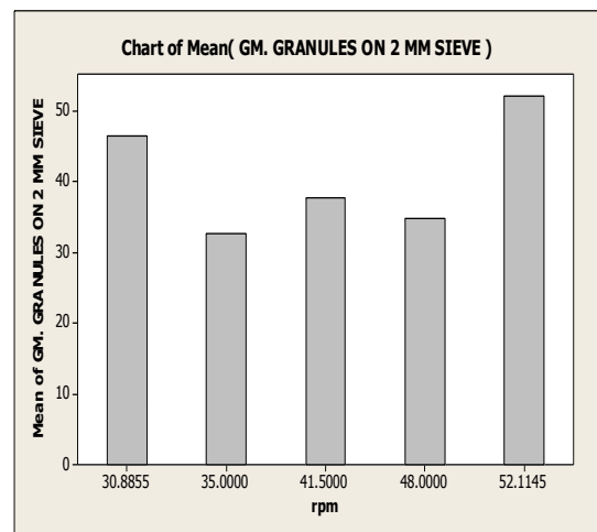
Fig.7 The relationship of rpm and percentage of 2mm granules obtained in IDG.
