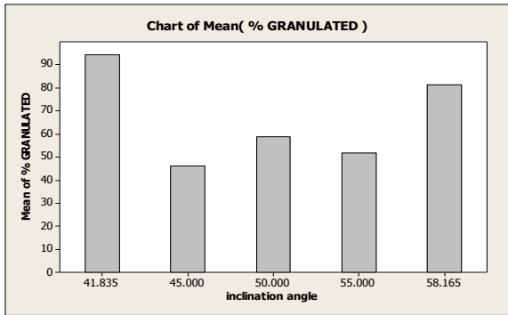
Fig. 2 The total percentage granulated with respect to angle of inclination in IDG.
