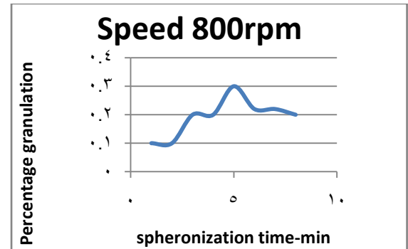
Fig. 15 spheronization of gamma alumina extrudate in Caleva spheronizer
