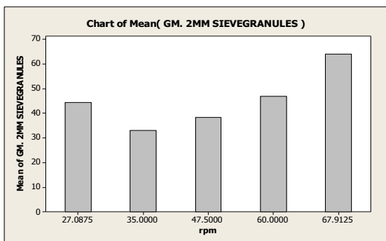
Fig.13 The relationship of speed to total granulation in the RD.
