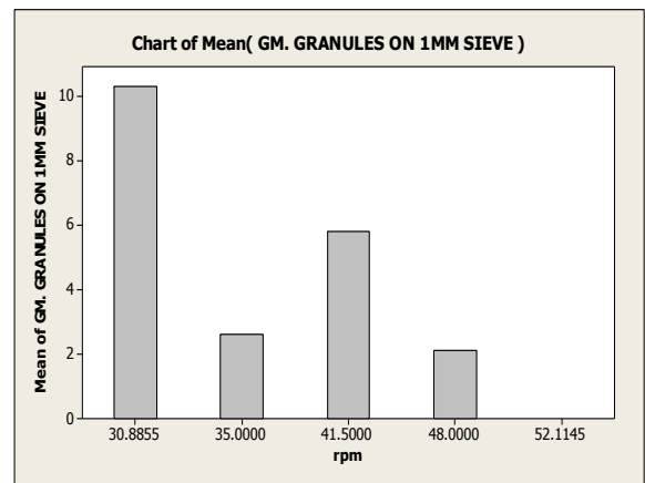
Fig. 6 Percentage of 1mm granulated with respect to speed of rotation.
