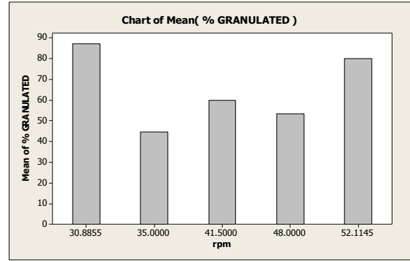
Fig. 5 The total granulated with respect to speed of rotation to IDG.
