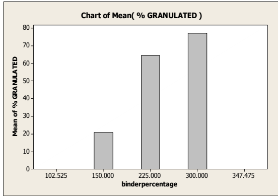
Fig. 8 The relationship between the binder percentage and percentage total granulation obtained in IDG.
