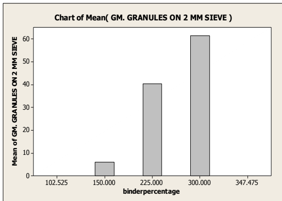
Fig. 9 the relationship between the binder percentage and percentage 2mm granules obtained in IDG.
