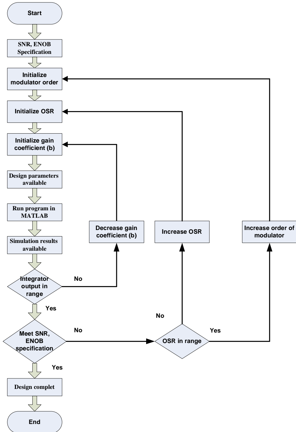
Figure (4): Flow chart of the simulation program.
