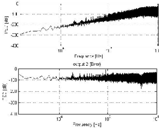
Figure(8): Simulation of quantization noise spectrum of the modulator ( y ) and in-band error quantization noise ( q(z) ).
