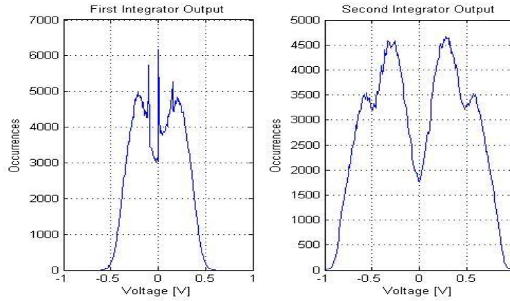
Figure (11): The output level histograms of the first and second integrators for proposed ADC.
