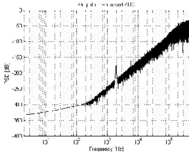
Figure (6): Simulation of quantization noise spectrum of the proposed novel ADC without decimation stage.
