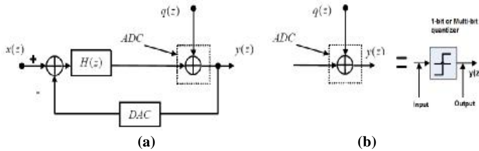
Figure 1): (a) First order oversampling ADC, (b) quantizer [5].
