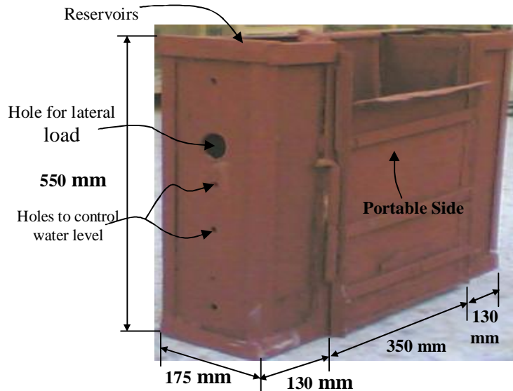
Figure (3): Steel container diagram
