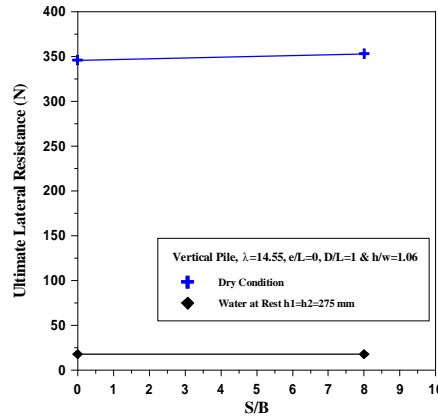
Figure (19): Comparison between results of ultimate lateral resistance of pile for dry and water at rest states.
