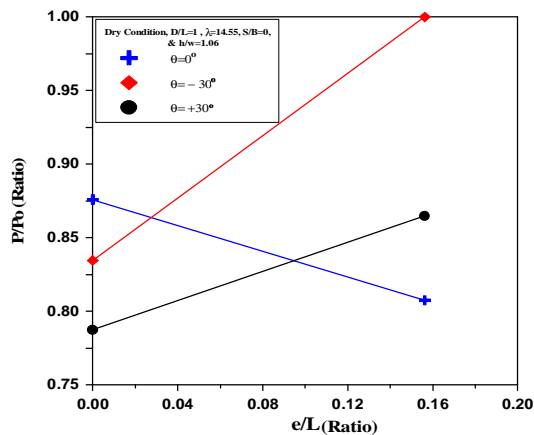
Figure (13): Ultimate lateral resistance (percent of no cavity condition) of pile versus pulling height ratio at various pile slope.
