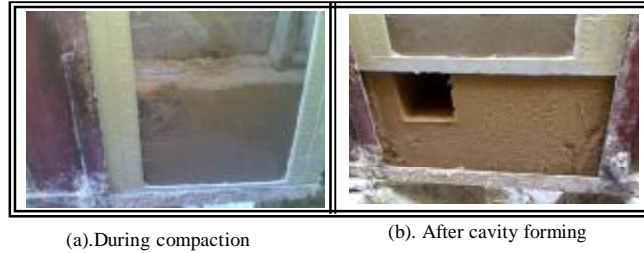
Figure (4): Stages for the preparation of the model test.
