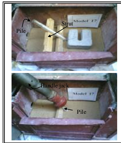
Figure (5): Methods of pile installation.
