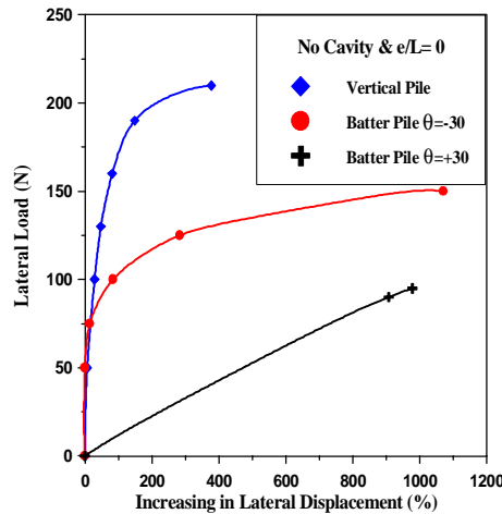
Figure (18): Relationship between lateral load and increasing in lateral displacement (due to the water presence).
