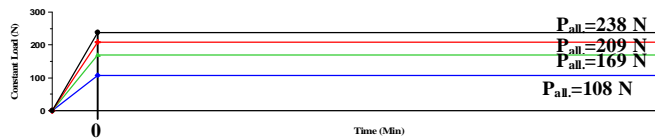
(a). lateral load versus time.
