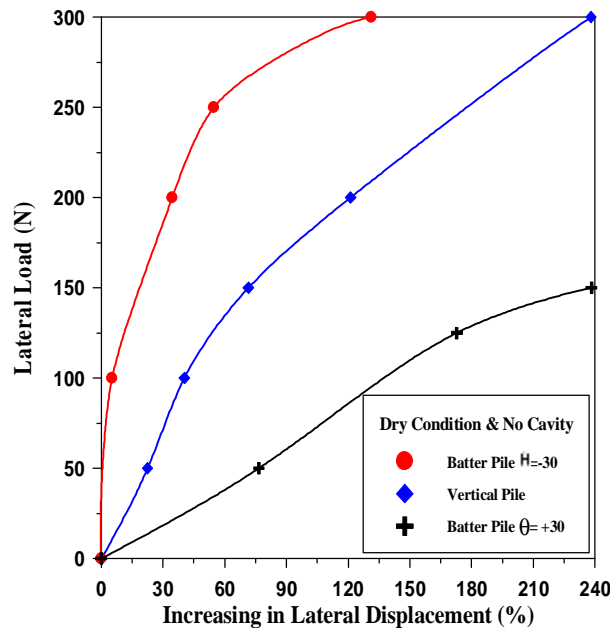
Figure (11) Model tests for no cavity condition.
