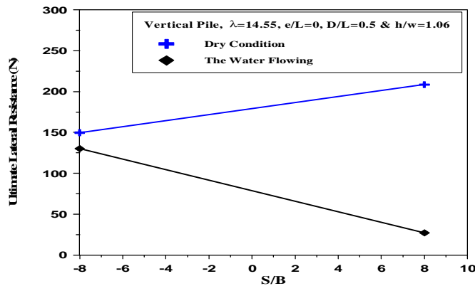
Figure (21): Relationship between lateral load at failure ( P_u ) and lateral distance ratio ( S/B ) for two different states.
