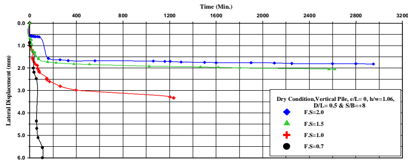
(b). Observed of surface lateral displacements with time due to the formation of the cavity under constant lateral loads
