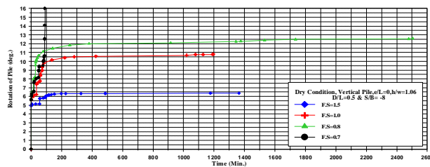
(c). Pile rotations versus time due to the forming of the cavity under constant lateral load
