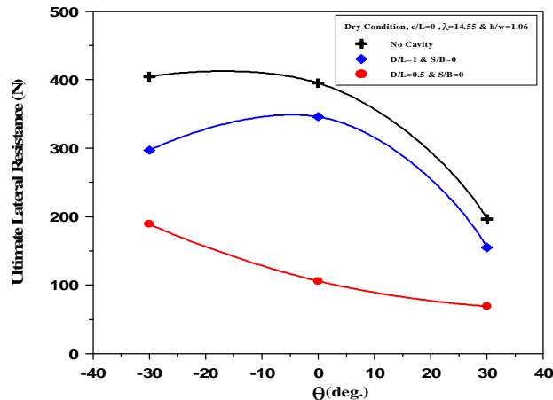
Figure (10): Effect of cavity depth ( D/L ) and pile inclination on ultimate lateral load resistance.
