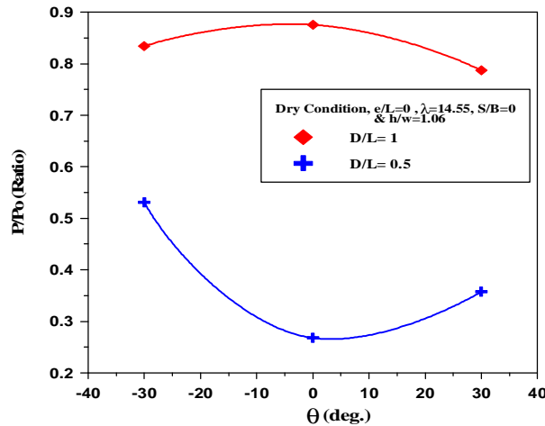
Figure (9): Relationship between reductions of ultimate lateral load resistance with pile slopes.
