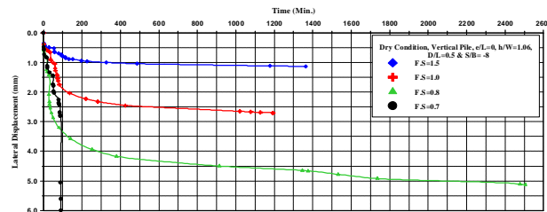
(b). Predicted lateral displacements at pile head due to the formation of the cavity versus time for different constants lateral loads
