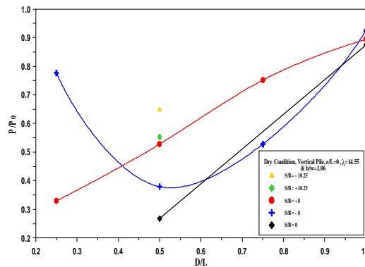
Figure (8): Effect of horizontal location and depth of cavity on ultimate lateral resistance.
