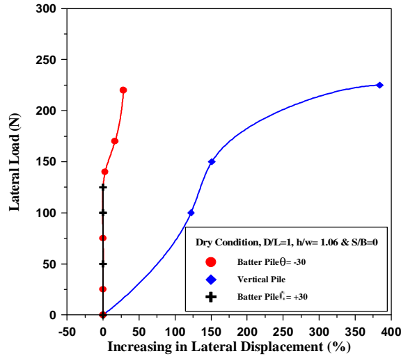
Figure (12) Model tests for cavity (D/L=1 and S/B=0).
