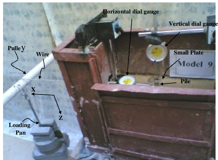
Figure (6): Experimental set-up
