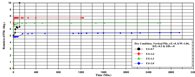
(c). Pile rotations with time due to the forming of the cavity under constant lateral loads
