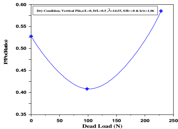
Figure (14): Relationship between reduction in ultimate lateral resistance of pile due to the cavity presence and vertical dead load.
