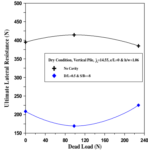
Figure (15) : The combined effect of vertical dead load and cavity presence on the ultimate lateral resistance of pile.
