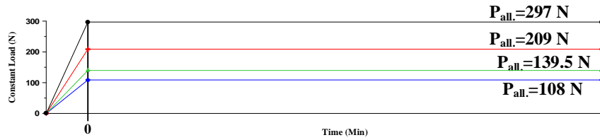
(a). Relationship between the lateral load and time
