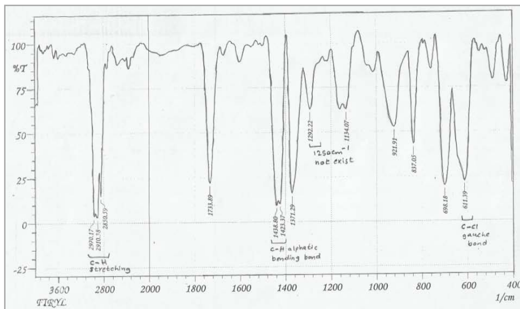
Figure 11 Infrared spectroscopy for commercials PVC, before Irradiation.
