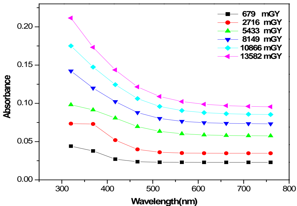
Figure 4 Absorbance difference as a function of Wavelength for PVC
