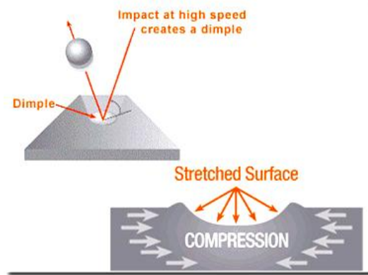
Figure (3) The surface after shot peening [18].
