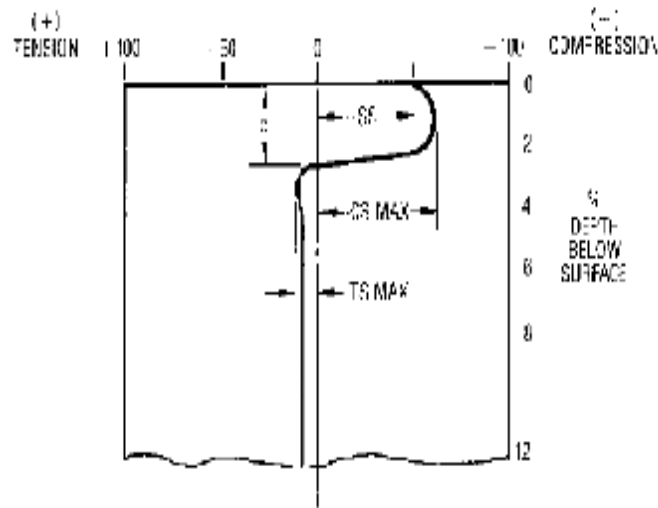
Figure (4) Residual stress after shot peening [19].
