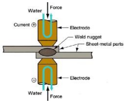
Figure (2) RSW configuration [17].
