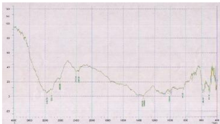
Figure (9) FTIR spectrums of CaP powder-untreated carbon fibers before heat treatment.
