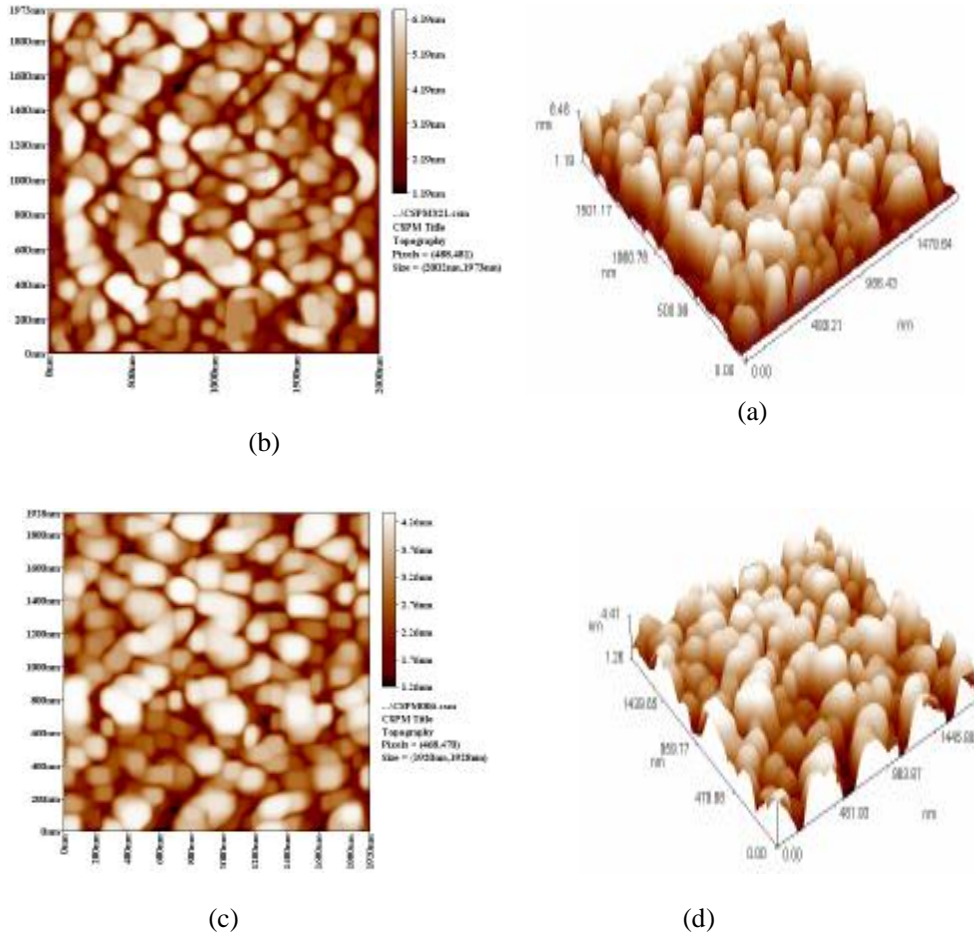
(c) (d) Figure (8) 2D & 3D AFM image for CaP coat (a,b) before heat treatment. (c,d) after heat treatment.
