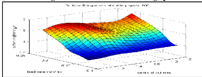
Figure (14) Surface roughness of insert 2 with cutting speed of 160 m/min
