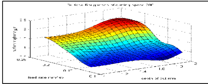
Figure (12) Surface roughness of insert 1 with cutting speed of 200 m/min Table (7) Optimum feed rate and depth of cut which give minimum surface roughness of each cutting speed for insert 1
