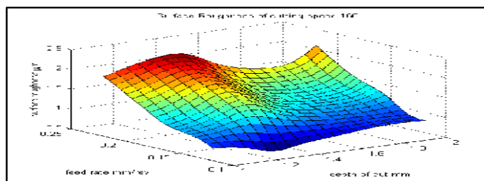
Figure (11) Surface roughness of insert 1 with cutting speed of 160 m/min
