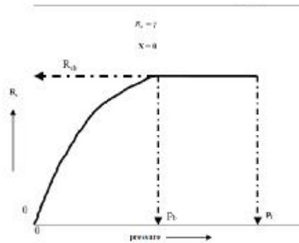
Figure (1): Typical gas solubility/pressure relationship (2) .
