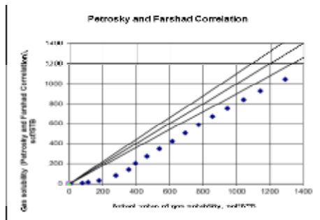
Figure (18): Cross Plot of Gas-oil ratio (Experimental data vs. the calculated data of Petrosky and Farshad's Correlation) for the external data.
