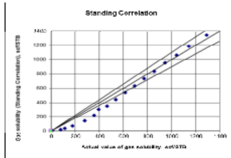
Figure (14): Cross Plot of Gas-oil ratio (Experimental data vs. the calculated data of Standing's Correlation) for the external data.
