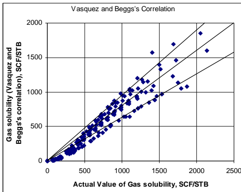
Figure (8): Cross Plot of Gas-oil ratio (Experimental data Versace the calculated data of Vasquez and Beggs's Correlation)
